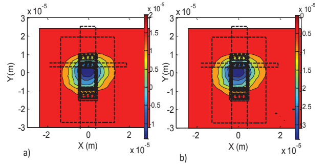
Figure 3: Base current mapping over the structure of the SiGe HPT. a) Phototransistor mode, b) Photodiode mode
