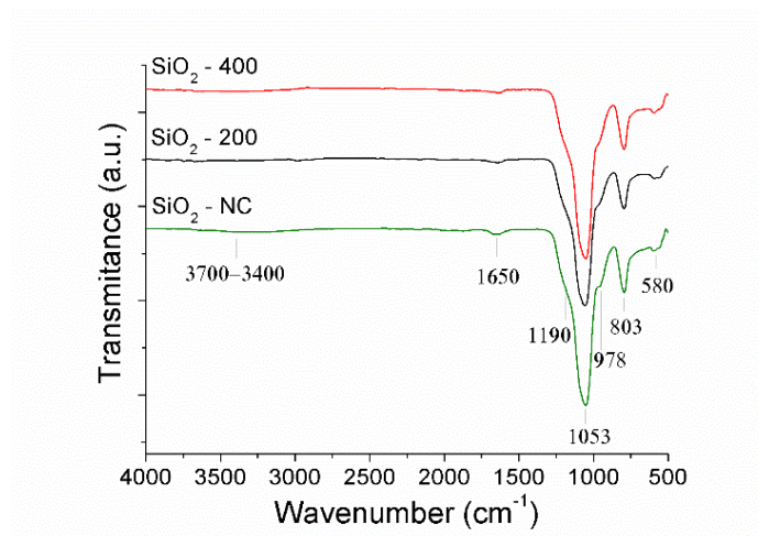
Fig. 3. Infrared spectra of the three starting silica nanoparticle samples
