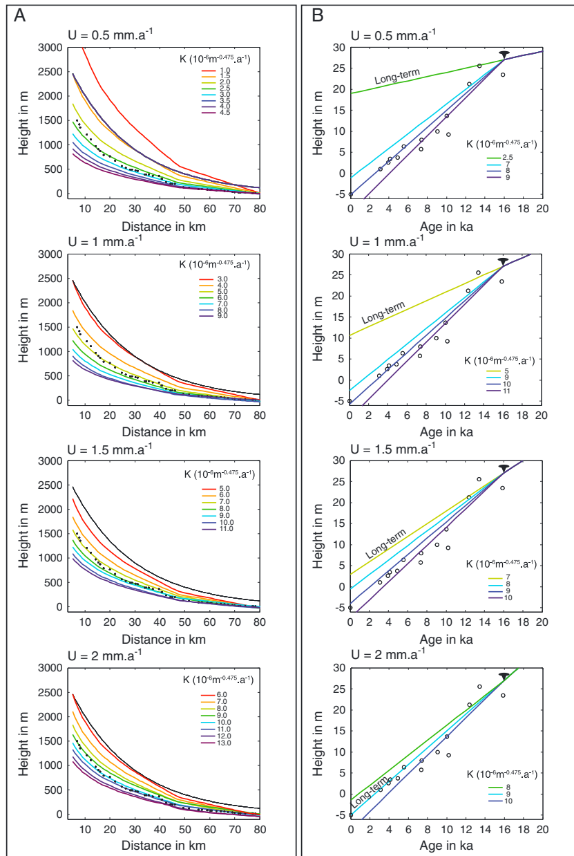
Figure 6. (a) Models of the equilibrium river profile (colored lines) with different K values for four different long-term uplift rates of 0.5 to 2 \text{mm a}^{-1} . Solid dots are measured altitudes along the river channel based on the SRTM digital elevation model. (b) Age/height relationships predicted at the sampling site for different long-term uplift rates and average short-term (16 ka) K values, including the long-term ones (best fitting curve on the corresponding Figure 6a). Open dots correspond to measured sample ages. Pinpoint at 16 ka, 26 m is indicated. Note that for every uplift rate lower than 2 \text{mm a}^{-1} , the average short-term (16 ka) K value is larger than the long-term one.
