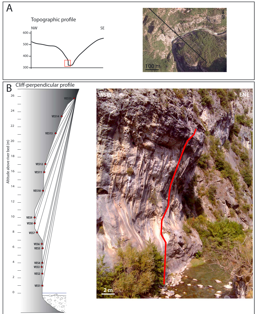
Figure 2. (a) Valley-perpendicular topographic profile and aerial view of the sampling site. Open red rectangle corresponds to the close-up view shown below. (b, left) Cliff-perpendicular topographic profile with altitudes relative to the present river bed. Red stars show the samples location. Thin lines are used to calculate the shielding effect of the overhanging cliff. Sample names are indicated in bold. (b, right) Picture of the polished river cliff. Red line indicates the approximate position of the sampled vertical profile.
