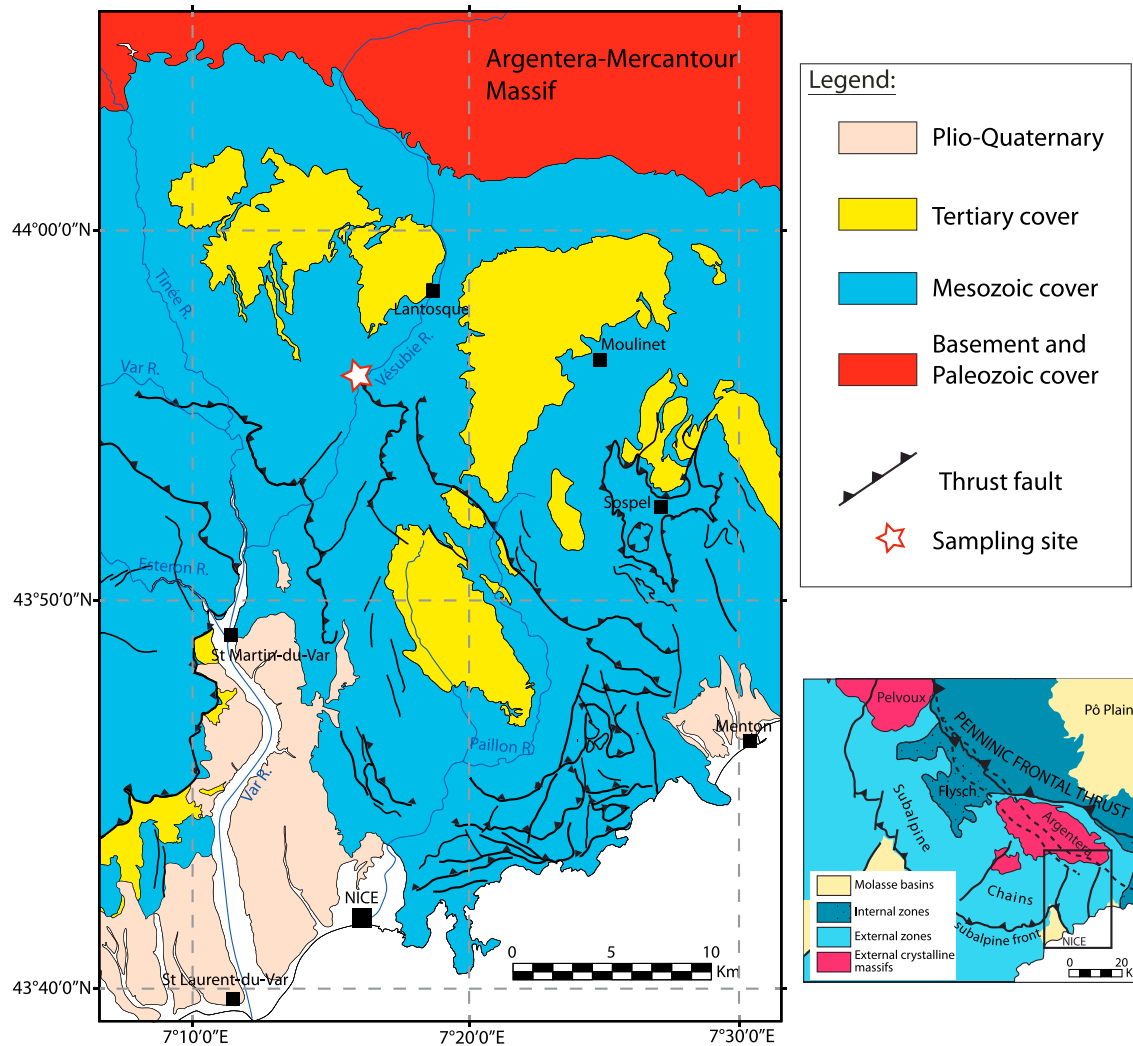
Figure 1. Geologic setting of the Vésubie and Var catchment areas. Southern French Alps [after Sanchez et al. , 2011]. Open red star shows the sample location. Inset shows the tectonic setting of the study area in the framework of the western Alps. Internal units consist of alpine metamorphic domains thrust over the external, nonmetamorphic basement and cover units.
