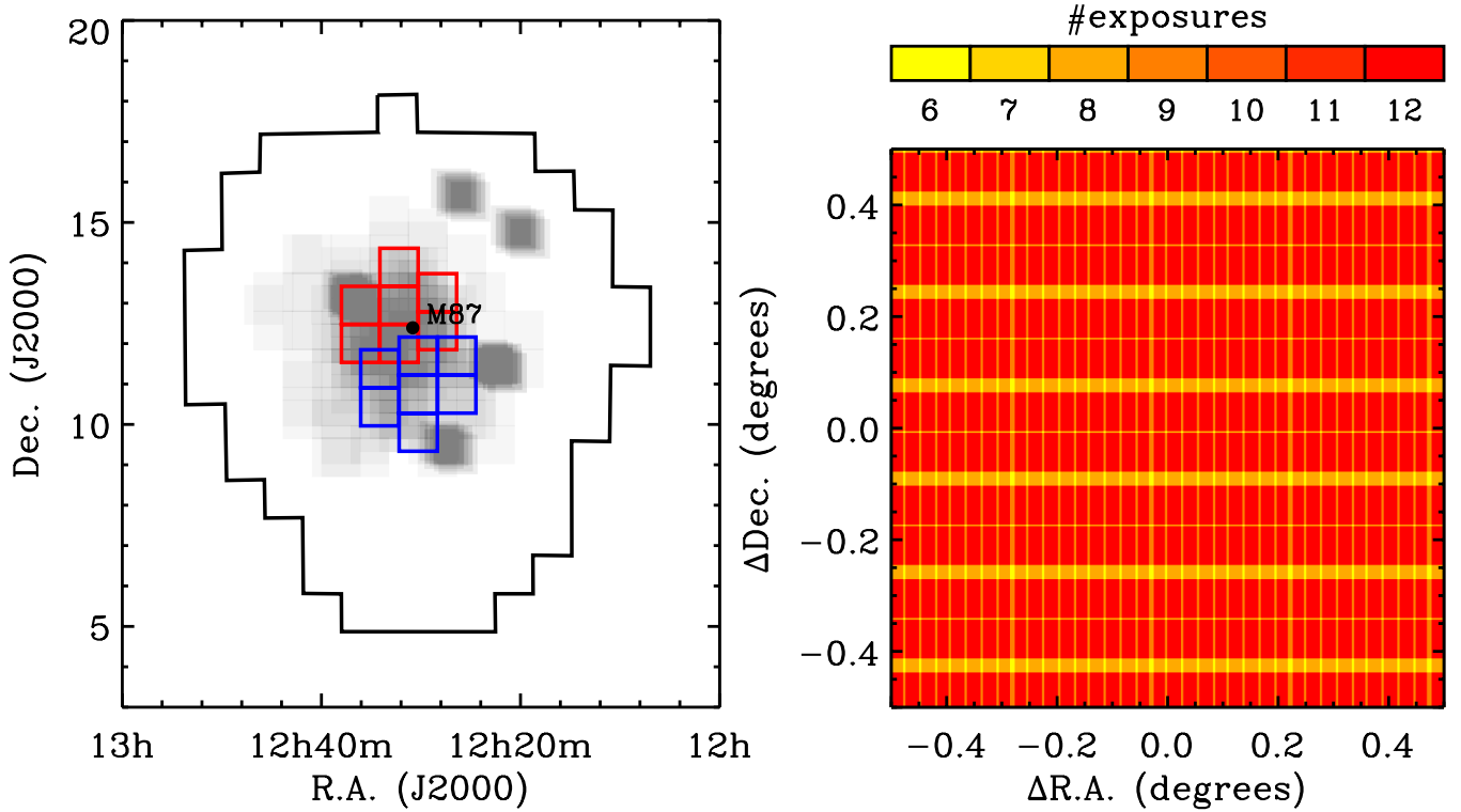
Fig. 5. Left: VESTIGE maps of the 104 \text{ deg}^2 within the NGVS footprint with 1419 independent frames in both the H\alpha NB and the r -band filters. To optimise the flat-fielding using the Elixir-LSB pipeline, the observations are gathered within an observing block of seven concatenated and adjacent frames, as depicted by the red and blue footprints here taken as two examples. The total number of observing blocks requested to cover the whole cluster is 203. Those obtained after the 2017A observing campaign are marked in grey with brightness increasing with the number of completed exposures (0 = white, 12 = dark grey). The dark regions in the outskirts of the clusters are the pilot observations completed in 2015 and 2016. Right: each sky region is covered by 12 independent frames dithered by 20 arcmin in right ascension (RA) and 15 arcmin in declination (Dec). This large dithering secures the sampling of the gaps between the different CCDs of MegaCam with a minimum of six exposures.
