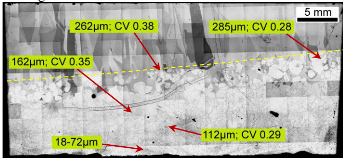
Fig. 4. Build-up of the same area as in Fig. 3 (optical images after chemical attack). The yellow dashed line delineates the initial growth interface determined from PL. Local grain size in genuine non-melted seed are also indicated.
