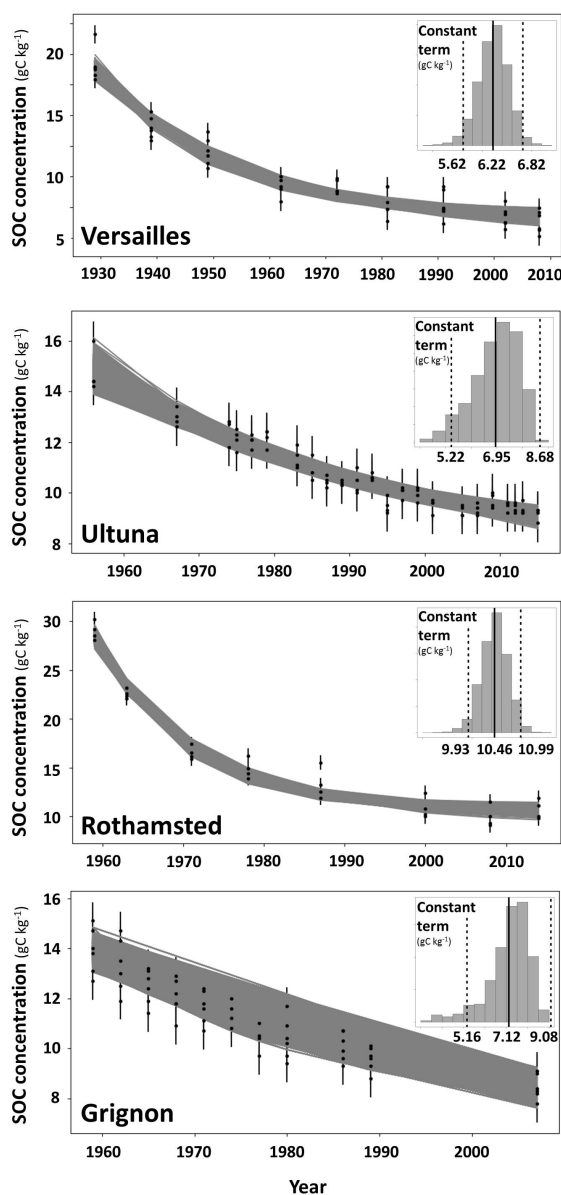
Figure 2. Evolution of SOC concentration (g C kg -1 of soil) with time for the bare fallow plots of each experimental site and representation of the 3 \times 10^4 fitted exponential decay functions (Bayesian curve-fitting method) from which a site-specific CP SOC concentration (model parameter c ) and its 95 % confidence interval were determined (histogram in the upper right corner of each scatter plot). At each site, the 95 % confidence interval around the CP SOC concentration was determined as c \pm 1.96 \text{ SD}(c) , where c is the model parameter c in Eq. (1) and \text{SD}(c) is its standard deviation.
