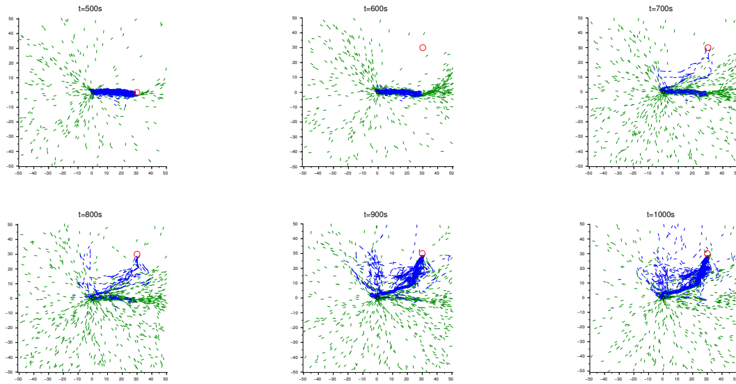
Figure 8: One simulation of the model with a dynamical food source. The food source is a disc of radius 2cm centered first at (30, 0) and then at (30, 30) after 500s. Green sticks: "green" pheromones. Blue sticks: "blue" pheromones. Red circle: food source. Black circle: nest.
