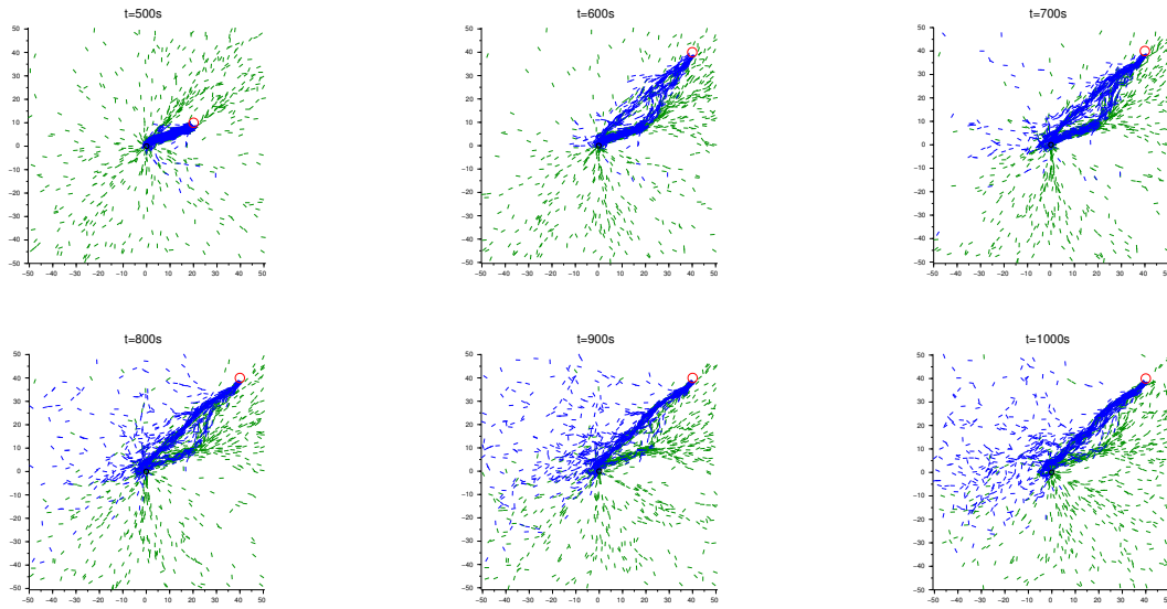
Figure 7: One simulation of the model with a dynamical food source. The food source is a disc of radius 2cm centered first at (20, 10) and then at (40, 40) after 500s. Blue sticks: "blue" pheromones. Green sticks: "green" pheromones. Red circle: Food source. Black circle: nest.
