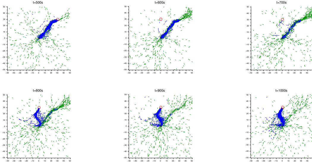
Figure 9: One simulation of the model with a dynamical food source. The food source is a disc of radius 2cm centered first at (30, 30) and then at (0, 30) after 500s. Blue sticks: "blue" pheromones. Green sticks: "green" pheromones. Red circle: Food source. Black circle: nest.
