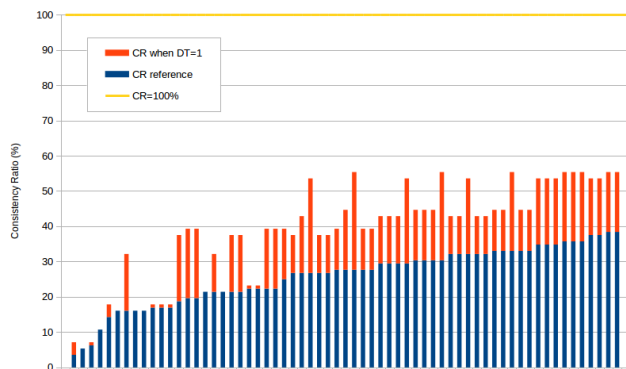
Fig. 4. Exhaustive CR analysis
