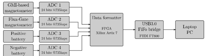
Fig. 2. Block diagram of the acquisition system.
