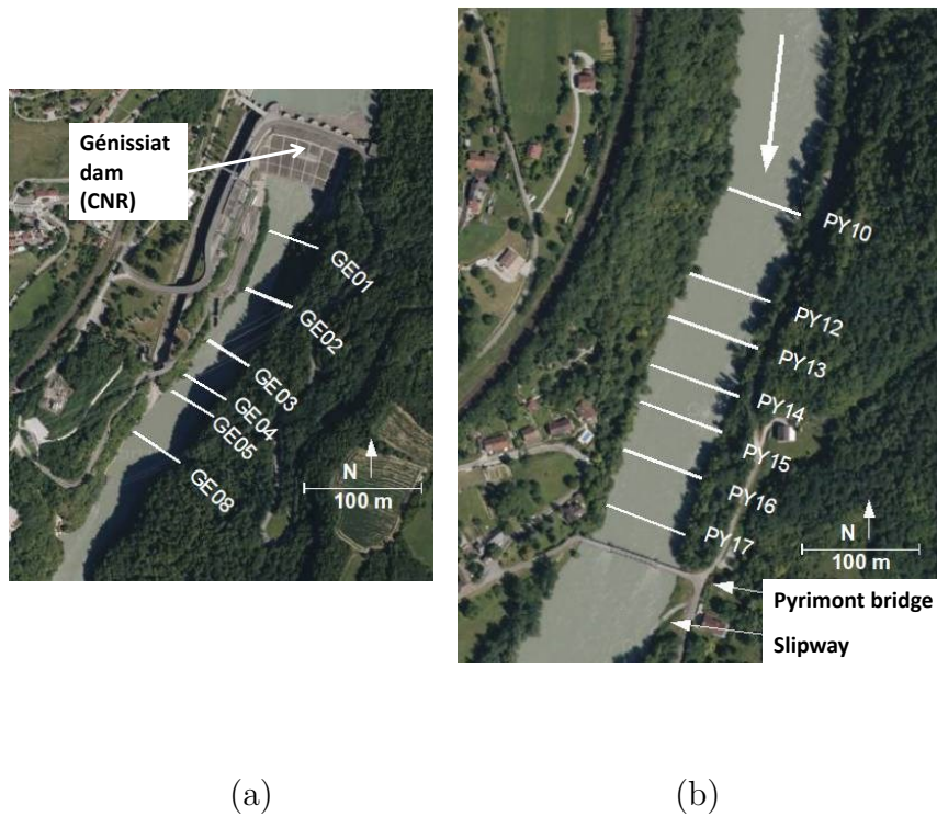
Figure 3: Aerial view of the ADCP transects at both sites of the Génissiat 2010 interlaboratory experiments: GE site downstream of the hydropower plant (a) and PY site upstream of the Pyrimont bridge (b). Modified from Google Maps (Map data © 2010 Google).
