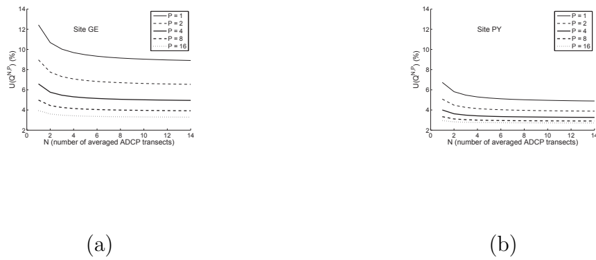
Figure 6: Expanded uncertainty in discharges measured as the average of N transects from P ADCP at both sites of the Génissiat 2010 interlaboratory experiments: GE site with adverse conditions (a) and PY site with favourable conditions (b). Expanded uncertainties are expressed with a probability level of 95%.
