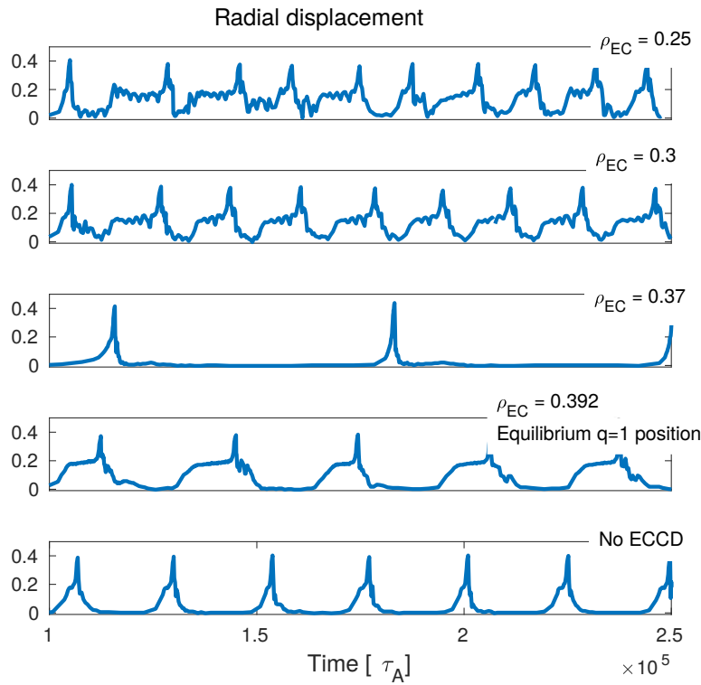
Figure 20. Evolution of the radial location of the maximum of the temperature as a function time, for different locations of the current deposition ( \alpha_{CD} = 1 , I_{RF}/I_P = 1\% ). One observes that depending on the location of the deposition, the radial trajectory of the hot core differs. In particular, for certain depositions, it features a long oscillatory period around \rho = 0.2 , that is, midway from its ejection value at \rho \approx 0.4 .
