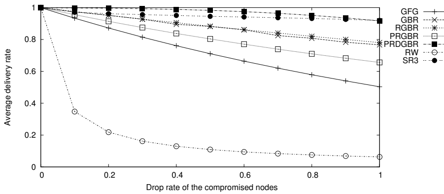
Fig. 13 Average delivery rate (20% of SF nodes, n = 200 , \bar{\delta} = 8 )
