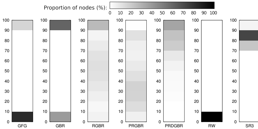
Fig. 16 Average delivery rate distribution (30% of BH, n = 200 , \bar{\delta} = 32 )
