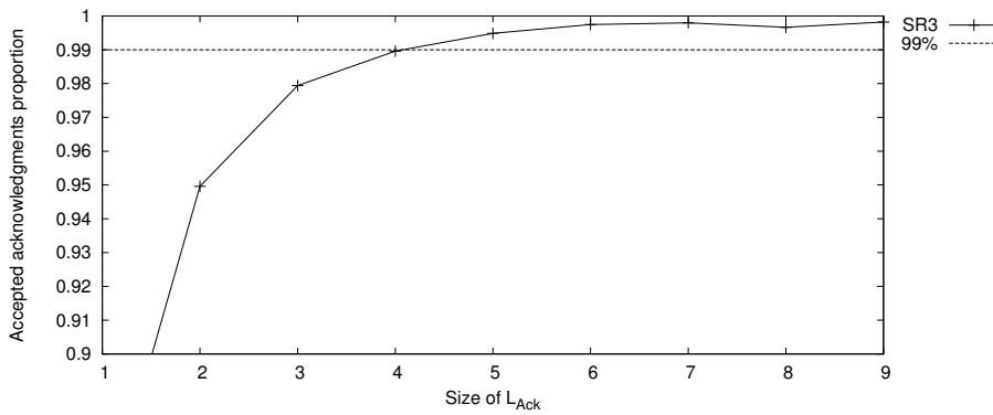
Fig. 8 Proportion of valid acknowledgments, depending on L_{AckRouting} size ( n = 200 and \delta = 8 )
