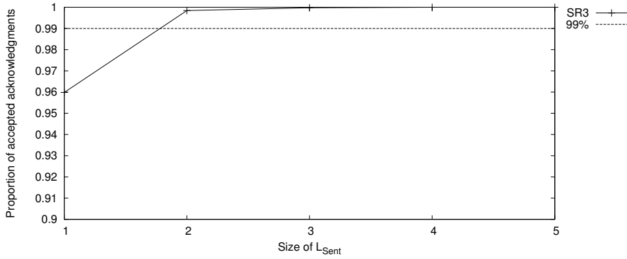
Fig. 7 Proportion of accepted acknowledgments, depending on L_{Sent} size ( n = 200 and \bar{\delta} = 8 )
