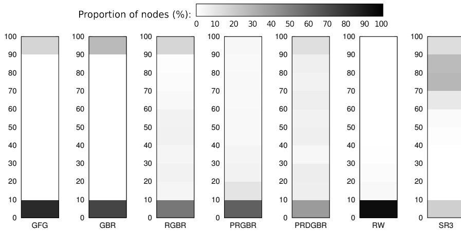
Fig. 17 Average delivery rate distribution (30% of BH, n = 200 , \bar{\delta} = 8 )
