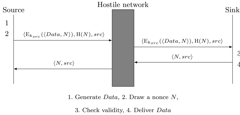
Fig. 4 Modeling of one session of SR3
