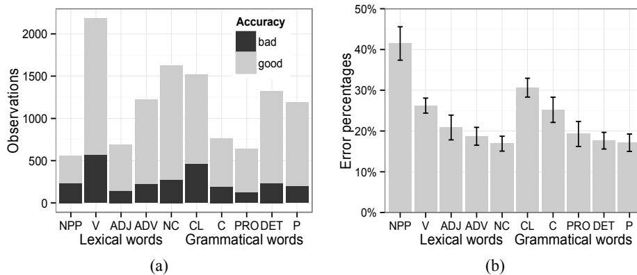
Figure 3. (a) Number of ASR errors according to POS categories. Lexical words: NPP = proper names, V= verbs, ADJ= adjectives, ADV = adverbs and NC = common names. Grammatical words: CL = weak clitics, C = coordinates and conjunctions, PRO = pronouns, DET = determiners, P = prepositions. (b) Relative error rates as a function of POS category.
