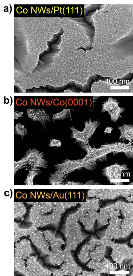
Figure 1. Scanning Electron Microscopy (SEM) micrographs of the surfaces of Co nanowire arrays grown on (a) Pt(111)/Al 2 O 3 (0001), (b) Co(0001)/Al 2 O 3 (0001) and (c) Au(111)/Cr/Si(001), after 24h of reaction (Co/LA/HDA ratio: 1/2/2, [Co] = 5mM, 24h, 150°C, solvent: anisole).
