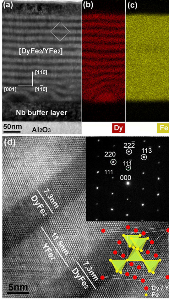
FIG. 2. (a) Low-magnification TEM image of the DyFe 2 /YFe 2 superlattice observed along the [1 \bar{1} 0] zone axis, (b) and (c) EDX elemental maps of Dy and Fe, and (d) high-resolution TEM image from the area marked by a square in (a), a diffraction pattern acquired along the [1 \bar{1} 0] zone axis, and a sketch of the unit cell of DyFe 2 (YFe 2 ) are given in the inset.
