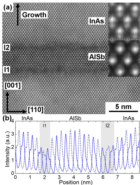
FIG. 1. (a) HAADF-STEM image along the [1\bar{1}0] zone axis of the InAs/AISb system. I1 and I2 refer to the interfaces. Insets are higher magnifications of the InAs and AISb layers. (b) Intensity line profiles along the growth direction taken in the middle of (a). Full and dotted lines come from two adjacent atomic rows.
