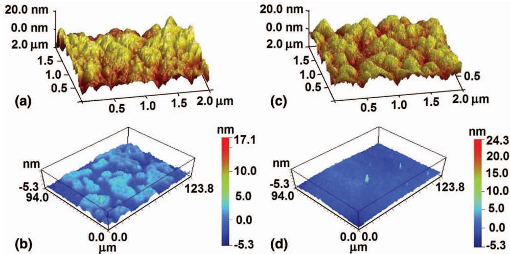
FIG. 2. Morphological properties of a NiFe/BF 3 (50 nm)/Co sample: a) & b) without AlO x ; c) & d) with AlO x ; by a) & c) AFM tapping mode, scan size 2 × 2 μm 2 and b) & d) Optical profilometer, scan size 124 × 94 μm 2 .
