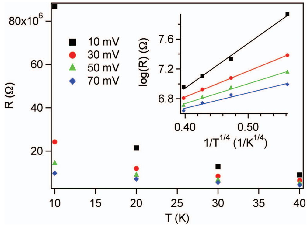
FIG. 5. Resistance versus temperature data for a NiFe/BF 3 (50 nm)/AlO x /Co sample and various applied voltages (Co anode). Inset : VRH fittings of these data (see text).
