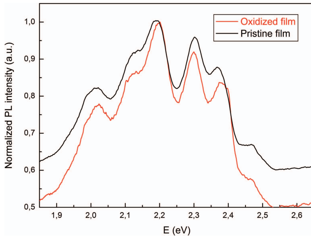
FIG. 6. Low temperature photoluminescence spectra of a pristine and an oxidized BF 3 film.
