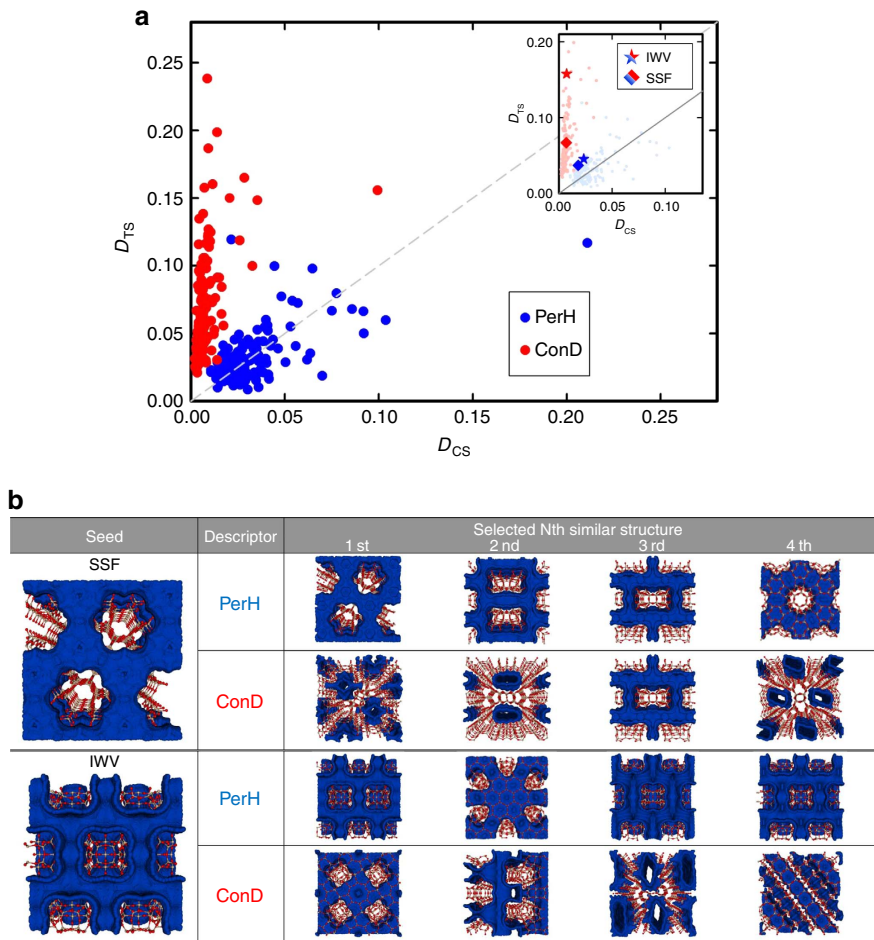
Figure 2 | Structures similar to a reference material. (a) For each known zeolite, the two sets of four most similar structures, once selected using the TDA descriptor (PerH, one blue dot for a set of four) and once selected by the conventional descriptor (ConD, one red dot per set) are compared. This is done by plotting their average distances D_{CS} in conventional space (x-axis) and their average distance D_{TS} in the barcode space (y axis) to the reference zeolite. The distances are normalized by the largest pairwise distance in the database. (b) The four structures most similar to the zeolite SSF respectively to IWV, as selected by either PerH or ConD. Their structural properties are given in Supplementary Table 1. The inset in a highlights the four sets of four structures shown in b .
