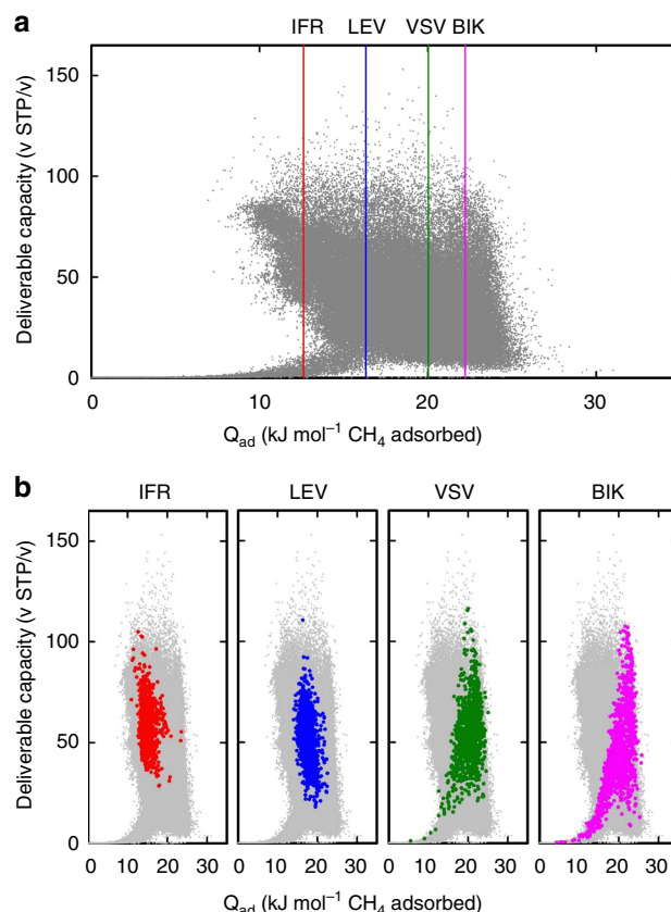
Figure 5 | The deliverable capacity and heat of adsorption of zeolites.
