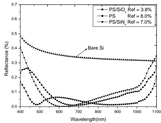
Figure 3 Reflectance spectra of PS/SiO x , PS/SiN x films on n+/p junction compared to as-grown PS.
