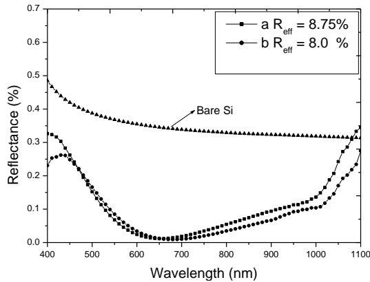
Figure 2 Total reflectance spectra of : (a) PS growth in HF (48 %): C_2H_5OH = 3:1 , J=20mA/cm^2 , t=6s ; (b) HF (48%): C_2H_5OH = 4:1 , J=20mA/cm^2 , t=6s .
