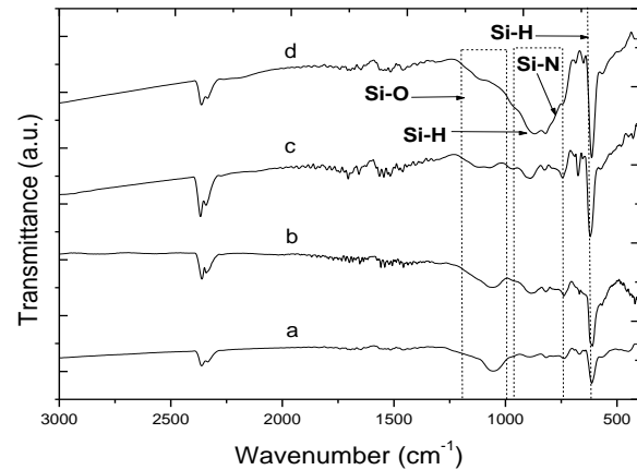
Figure 5 FTIR transmission spectra of structure (a) PS/ \text{SiO}_x , (b) PS after annealing, (c) PS, (d) PS/ \text{SiN}_x\text{:H} .
