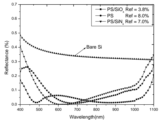
drogen in the SiN x :H layers: H diffuses within the thin Figure 3 Reflectance spectra of PS/SiO x , PS/SiN x films on n+/p junction compared to as-grown PS.
