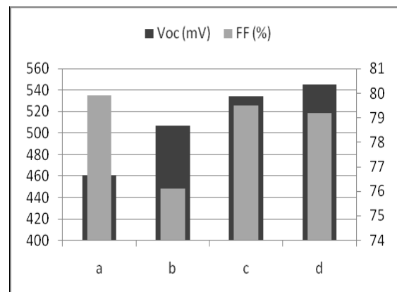
Figure 4 Parameters suns- V_{oc} obtained in a junction respectively before and after RTA with PS before (a) and after (b) annealing. (c) PS/SiO x , (d) PS/SiN x .
