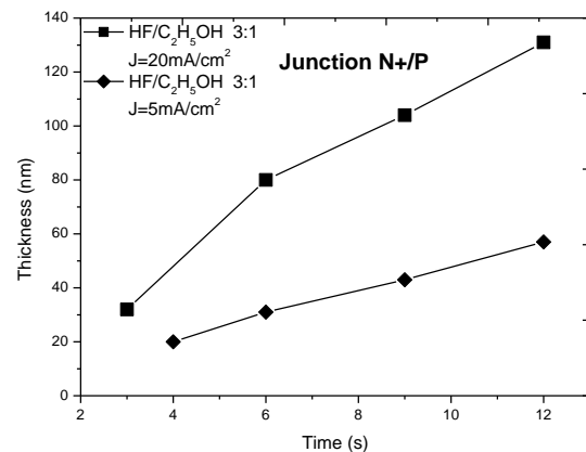
Figure 1 Thickness E vs time t of PS growth at a constant current density of 5\text{mA}/\text{cm}^2 and 20\text{mA}/\text{cm}^2 on n^+ diffused side of (100) Si wafer.
