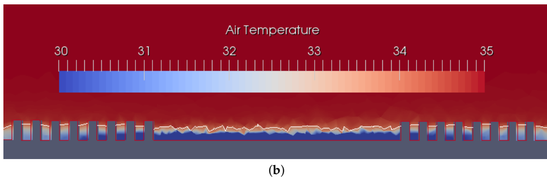
Figure 11. Vertical slice of the air temperature field for a low building density district. (a) UF 1: buildings are 10 m high; (b) UF 6: buildings are 17 m high—the white line is the 34 °C isotherm.
