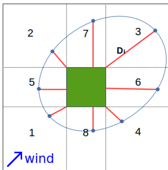
Figure 3. Zoning (dashed lines and numbers) and example of calculation (red lines) used to calculate the distance between any point on the 34 °C isotherm and the park boundary.
