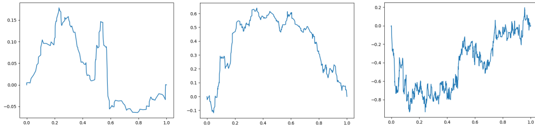
(B) E-LPP for m = 10^4 with b = 0 and from left to right a = 1, a = 4/3, a = 2 ; corresponding to \kappa = 1/2, \kappa = 4/7, \kappa = 2/3 . From left to right \mathcal{L}_m = 150, \mathcal{L}_m = 303, \mathcal{L}_m = 690 ; the ratio \mathcal{L}_m/m^\kappa is approximately equal to 1.5, 1.57, 1.49 respectively. For 100 simulations, the mean value of \mathcal{L}_m/m^\kappa is 1.54, 1.59, 1.52 respectively.
