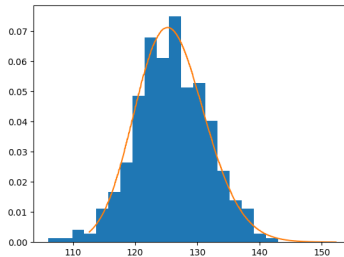
FIGURE 8. Histogram of 400 realizations of \mathcal{L}_m for m = 10^4 (still t, x, B set to 1), with a = 2, b = 1 ( \kappa = 1/2 ). We also plotted the graph of the GUE density, properly centered, and rescaled by cm^{\kappa/3} with c \approx 1.35 .
