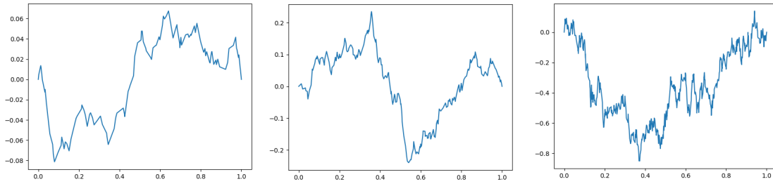
(A) E-LPP for m = 10^4 with b = 1 and from left to right a = 2, a = 8/3, a = 4 ; corresponding to \kappa = 1/2, \kappa = 4/7, \kappa = 2/3 . From left to right \mathcal{L}_m = 121, \mathcal{L}_m = 241, \mathcal{L}_m = 586 ; the ratio \mathcal{L}_m/m^\kappa is approximately equal to 1.21, 1.25, 1.26 respectively. For 100 simulations, the mean value of \mathcal{L}_m/m^\kappa is 1.26, 1.29, 1.29 respectively.
