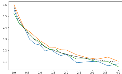
FIGURE 7. Simulations for the E-LPP (with t, x, B = 1 ) for m = 10^4 , for different values of b , with a adjusted to keep constant \kappa = 1/2 ( a = b + 1 ), \kappa = 4/7 ( a = 4(b + 1)/3 ) and \kappa = 2/3 ( a = 2(b + 1) ). For each value of b we took the mean value of \mathcal{L}_m/m^\kappa over 10 simulations, and the graphs represents this mean value as a function of b (with \kappa kept constant), as an approximation of c_b : the three graphs correspond to \kappa = 1/2 , \kappa = 4/7 and \kappa = 2/3 , and they appear to be relatively close. We observe that the function decreases to 1 as b increases – as a side note, we noticed that the function b \mapsto 2^{\frac{2}{3(b+1)}} (appearing as a dotted line) fits the plots quite well.
