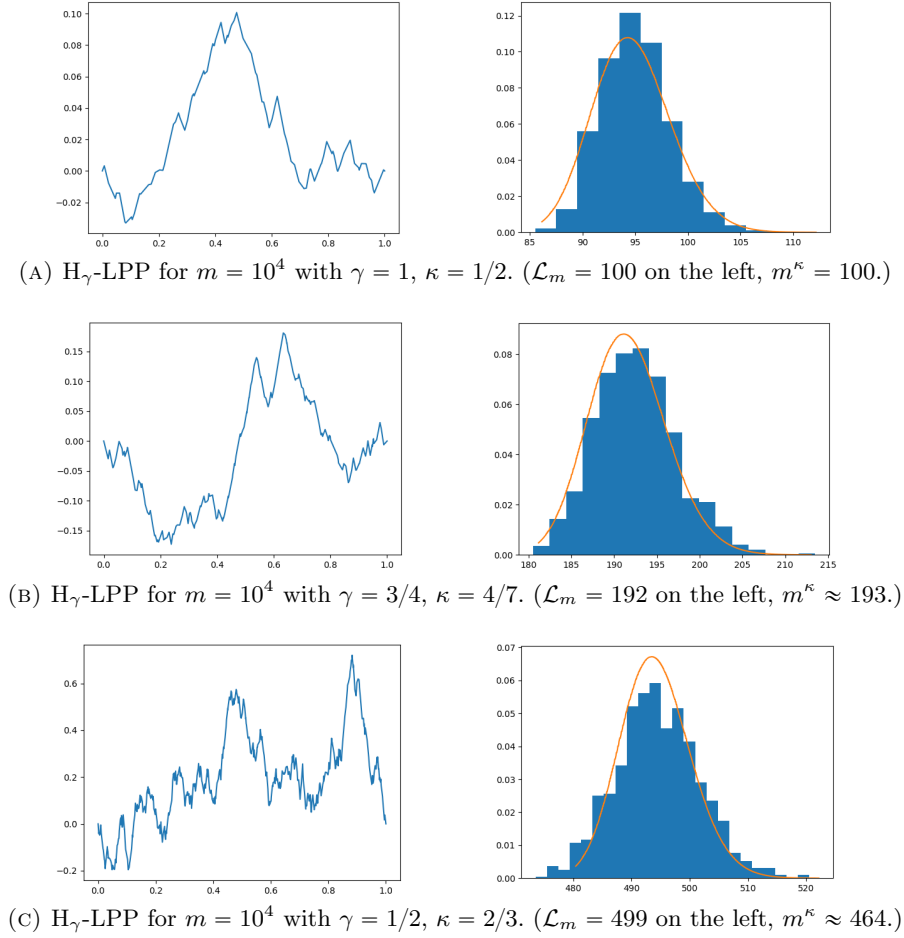
FIGURE 5. Exact simulation of point-to-point H_\gamma -LPP with t, x, A = 1 and m = 10^4 (intensity of points \lambda = m/2 ), and with \gamma = 1 , \gamma = 3/4 , \gamma = 1/2 in subfigures (A), (B), (C) respectively. In each case, we present: on the left a realization of a maximal path (with \mathcal{L}_m given in the caption of each figure); on the right, a histogram of k = 10^3 realizations of the H_\gamma -LPP, together with the graph of the Tracy-Widom GUE density (after a recentering by m^\kappa + cm^{\kappa/3} , and a renormalization by (m/2)^{\kappa/3} ).
