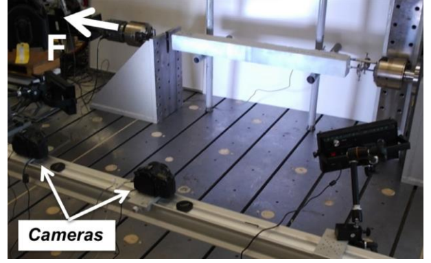
Figure 2: RC tie in tension: experimental set up.
