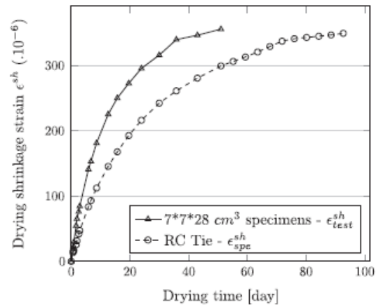
Figure 6: Drying shrinkage strain imposed to the structure.
