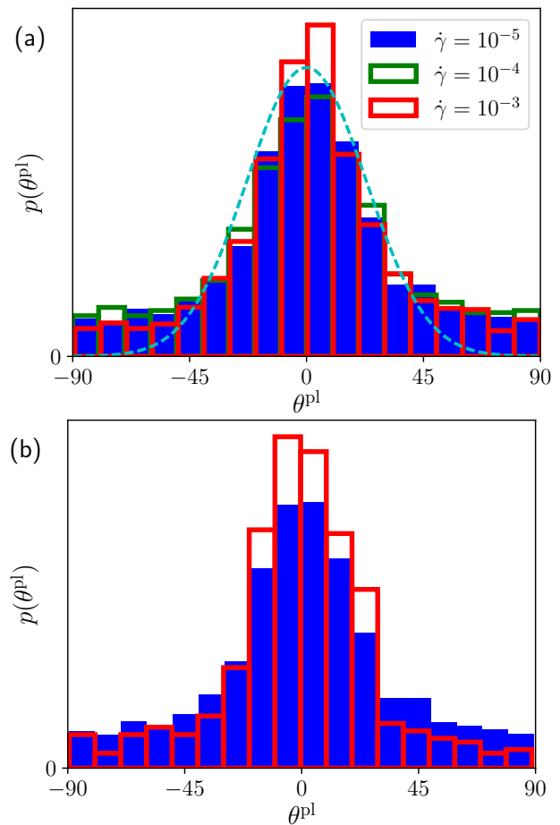
Figure 6. Distributions of angles of failure \theta^{\text{pl}} obtained with the MD/Esh method. (a) Comparison of p(\theta^{\text{pl}}) between distinct shear rates \dot{\gamma} . The dashed line represents a normal distribution with standard deviation \delta \theta^{\text{pl}} = 23^\circ . (b) Distribution p(\theta^{\text{pl}}) at \dot{\gamma} = 10^{-5} before (filled blue) and after (red) removing the STs which substantially deviate from their Eshelby fits ( \chi^2 > 0.5 ).
