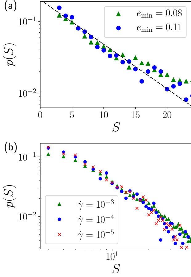
Figure 3. Distribution of sizes S of the rearranging clusters detected with the kinetic energy based criterion (a) for two different threshold values e_{\min} at \dot{\gamma} = 10^{-5} and (b) for three different shear rates \dot{\gamma} with e_{\min} = 0.11 . The thin dashed line in the top panel is proportional to \exp(-S/S_0) with S_0 = 7 .
