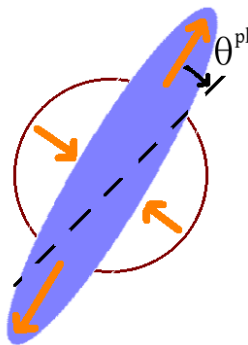
Figure 2. Representation of the angle of failure \theta^{\text{pl}} . The orange arrows indicate the elongational and contractive directions of an ideal ST, while the dashed line represents the elongational direction of the macroscopic shear.
