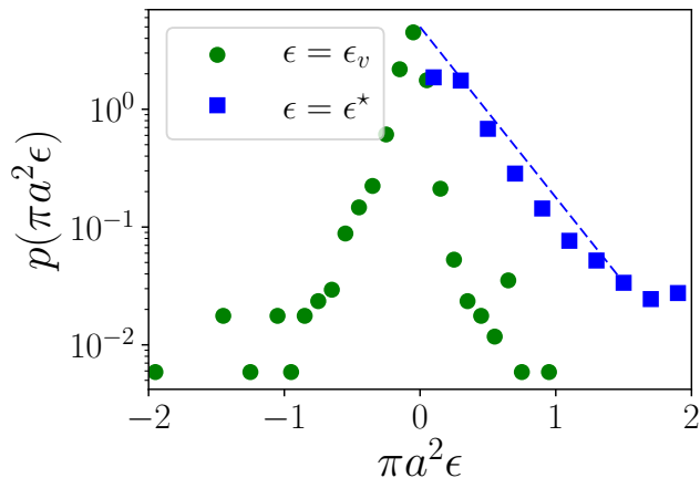
Figure 5. Distribution of the dilational strengths \pi a^2 \epsilon_v (circles) and the shear strengths \pi a^2 \epsilon^* (squares) of the STs detected at \dot{\gamma} = 10^{-5} (with threshold e_{\min} = 0.11 ). The dashed blue line is proportional to \exp(-x/0.3)
