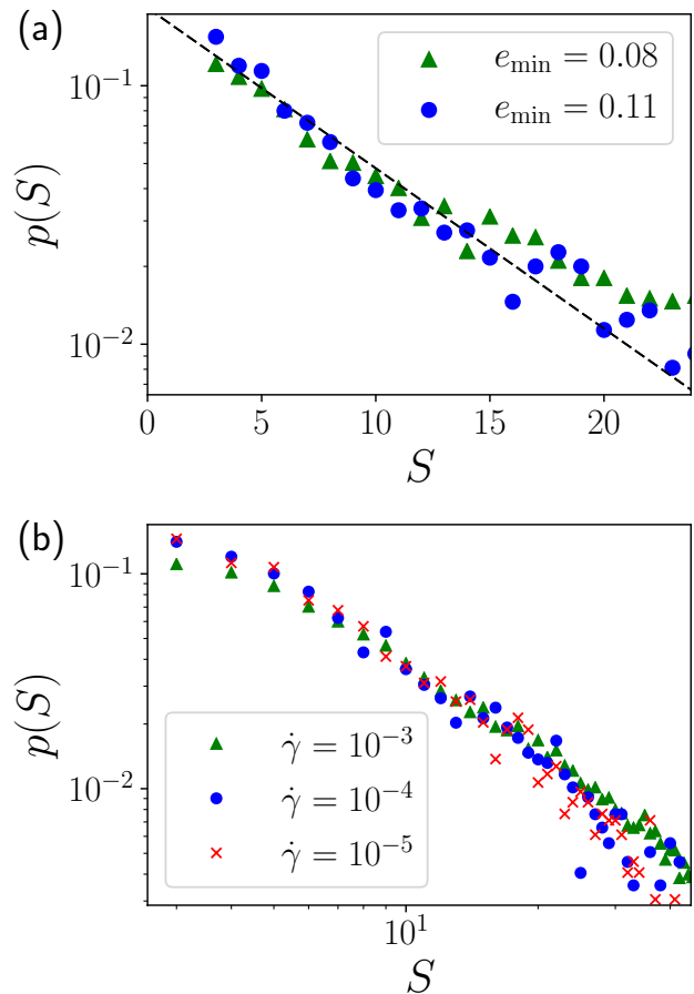
Figure 3. Distribution of sizes S of the rearranging clusters detected with the kinetic energy based criterion (a) for two different threshold values e_{\text{min}} at \dot{\gamma} = 10^{-5} and (b) for three different shear rates \dot{\gamma} with e_{\text{min}} = 0.11 . The thin dashed line in the top panel is proportional to \exp(-S/S_0) with S_0 = 7 .
