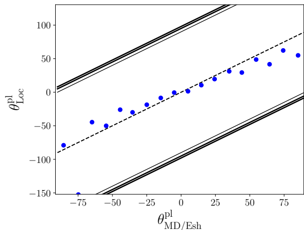
Figure 8. Comparison between the angles of failure \theta_{\text{MD}/\text{Esh}}^{\text{pl}} and \theta_{\text{Loc}}^{\text{pl}} measured with the MD/Esh method and the displacement-based local method, respectively. The STs have been binned into 10^\circ -wide angular windows, according to the value of \theta_{\text{MD}/\text{Esh}}^{\text{pl}} .
