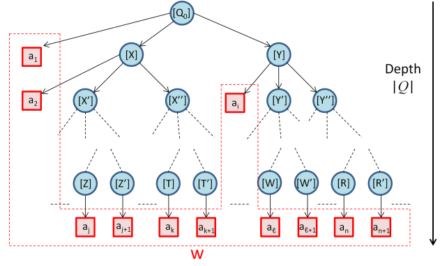
Fig. 3. Derivation tree of a word corresponding to a feasible path.
