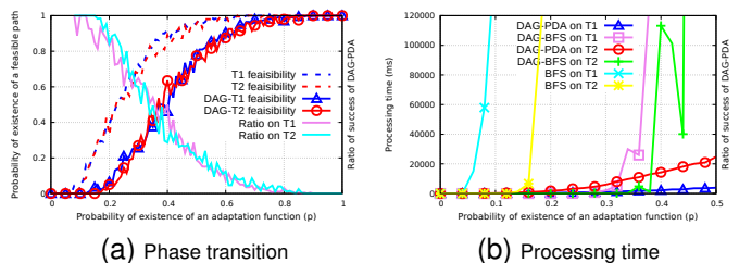
Fig. 9. Phase transition (before and after DAG conversion) and comparison of the processing time of DAG-PDA, DAG-BFS and BFS.
