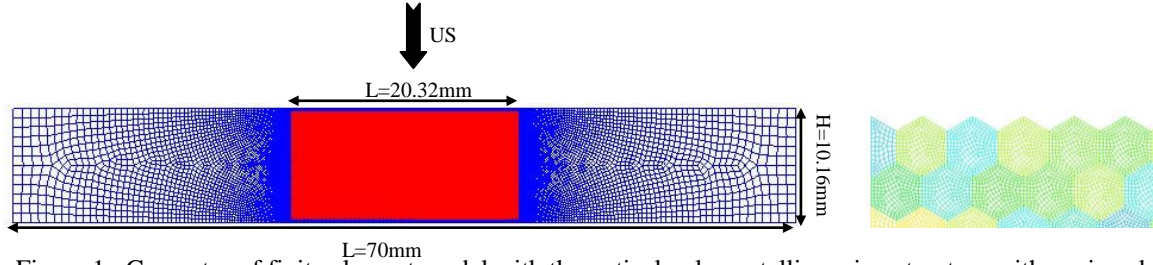
Figure 1 –Geometry of finite element model with theoretical polycrystalline microstructure with equiaxed hexagonal grains
