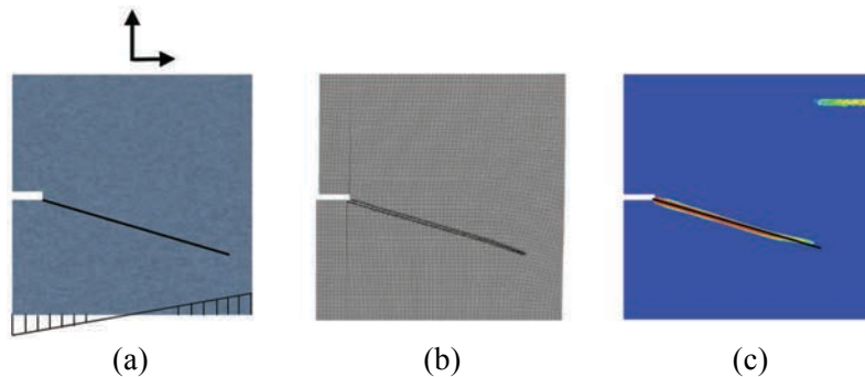
Fig. 2 Virtual hybrid test results for an imposed straight crack path: (a) imposed cracked path, (b) X-FEM results, (c) damage model crack path confronted with the desired trajectory.
