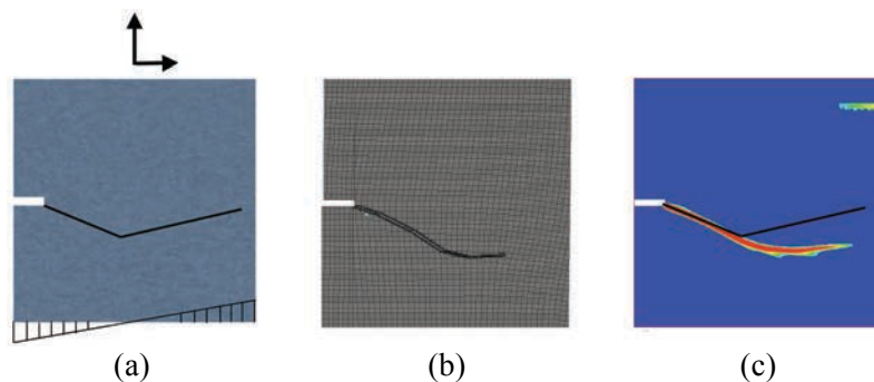
Fig. 3 Virtual hybrid test results for a more complex imposed crack path: (a) imposed cracked path, (b) X-FEM results, (c) damage model crack path confronted with the desired trajectory.
