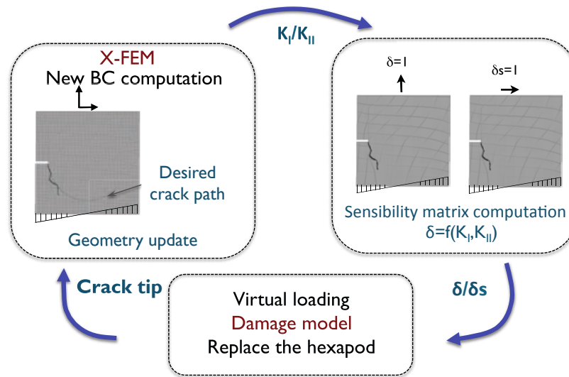
Fig. 1 Virtual hybrid test principle
