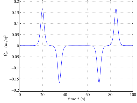
FIG. 11: The second derivative \ddot{V}_{xr} = \ddot{\Omega}_{\mathbf{p}_u, \mathbf{p}_d} (jerk).
