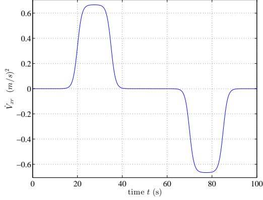
FIG. 10: The first derivative \dot{V}_{xr} = \dot{\Omega}_{\mathbf{p}_u, \mathbf{p}_d} (acceleration).
