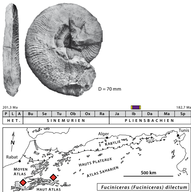
Fig. 188: Fucinicerus (Fucinicerus) dilectum (Fucini, 1900), D = 70 mm, Djebel Bou-Rharraf [Du Dresnay, 1963, pl. 1, fig. 3, modifié].
