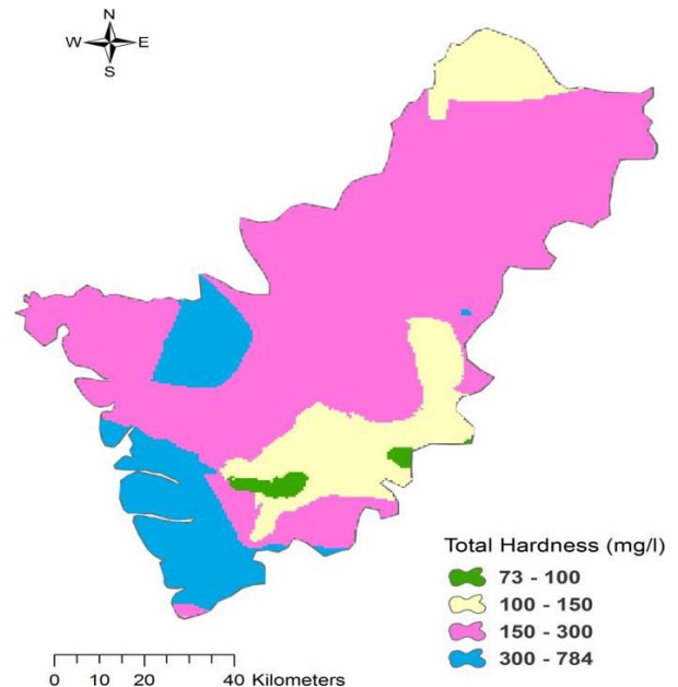
FIG. 8. SPATIAL DISTRIBUTION OF TOTAL HARDNESS IN THE STUDY AREA
