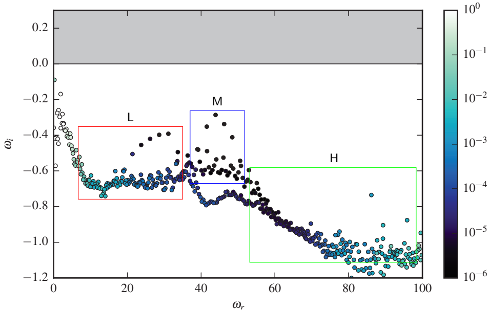
FIGURE 2. Global spectrum of the tonal noise problem in the complex frequency plane. The eigenvalues are colored according to the size of the relative residual with respect to the operator \mathbf{A} . The spectrum is divided into least stable modes (labelled M), low-frequency modes (labelled L) and high-frequency modes (labelled H).
