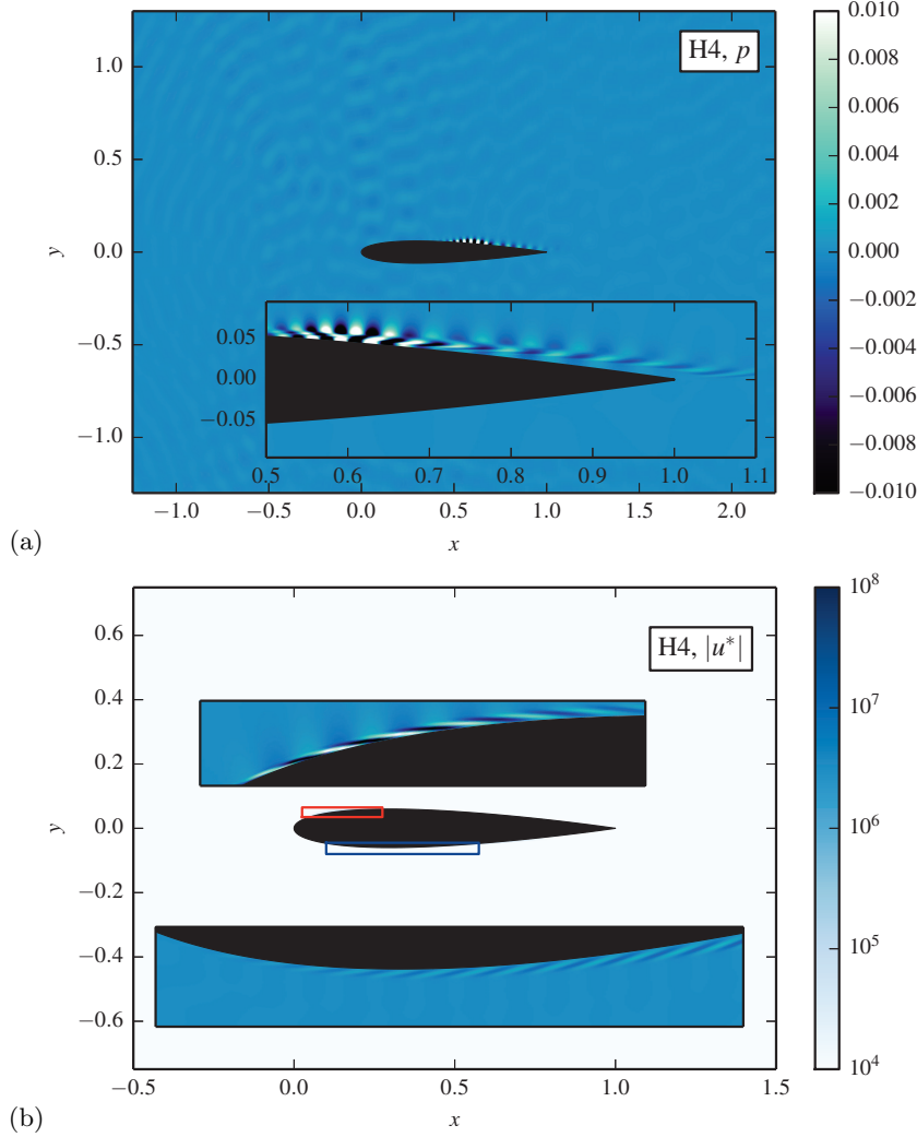
FIGURE 7. Direct and adjoint global mode corresponding to H_4 indicated in figure 6, visualised by the real part of the pressure field (a) and absolute value of the adjoint streamwise velocity (b). The insets, showing the real part of the streamwise velocity, give more details of the respective flow fields.
