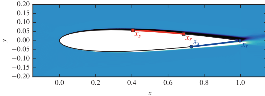
FIGURE 1. Mean flow considered in the present study, visualised by the streamwise velocity component. The boundary layer on the suction surface detaches between x_s \approx 0.405 and x_r \approx 0.686 , while the pressure-surface boundary layer detaches between x_s \approx 0.728 and x_r \approx 0.977 . The reader is referred to Fosas de Pando et al. (2014) for further details on the mean-flow characteristics.
