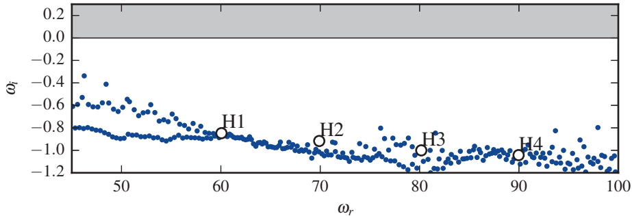
FIGURE 6. Global spectrum displaying high-frequencies \omega > 45 ; the modes labelled H_1 - H_4 will be analysed further. Their associated eigenfrequencies are: \omega_{H_1} = 60.06 - 0.85i , \omega_{H_2} = 69.90 - 0.92i , \omega_{H_3} = 80.17 - 1.00i , \omega_{H_4} = 89.97 - 1.05i . The residual associated with the iterative eigenvalue solver is smaller than 5 \cdot 10^{-3} .
