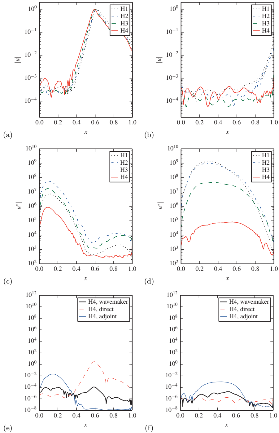
FIGURE 8. Evolution of the streamwise velocity peak along the aerofoil chord (a) on the suction- and (b) on the pressure surface of the aerofoil for the high-frequency modes labelled H_1 - H_4 in figure 6. (c,d) Same for the adjoint streamwise velocity peak. (e,f) Same for the direct mode, adjoint mode and wavemaker corresponding to H_4 .
