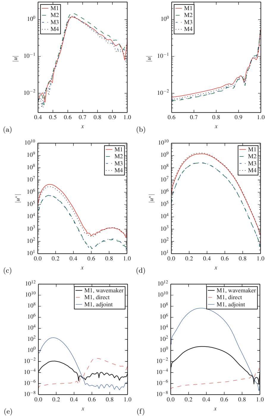
FIGURE 5. Evolution of the streamwise velocity peak along the aerofoil chord (a) on the suction- and (b) on the pressure surface of the aerofoil for the leading modes labelled M_1 - M_4 in figure 3. (c,d) Same for the adjoint streamwise velocity peak. (e,f) Same for the direct mode, adjoint mode and wavemaker corresponding to M_1 .
