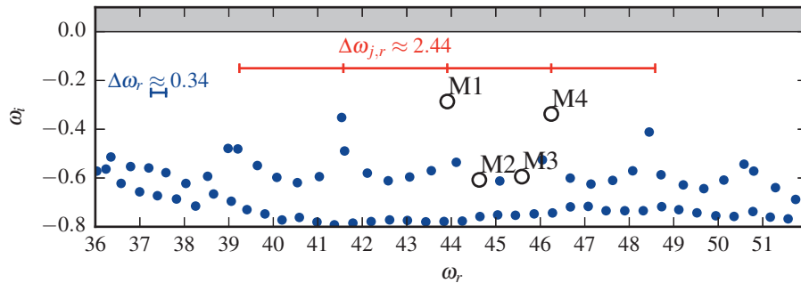
FIGURE 3. Zoomed view of the global spectrum showing the least stable (or leading) global modes. The modes M_1 - M_4 are considered in more detail, and the corresponding eigenvalues are \omega_{M1} \approx 43.91 - 0.29i , \omega_{M2} \approx 44.63 - 0.61i , \omega_{M3} \approx 45.59 - 0.59i and \omega_{M4} \approx 46.25 - 0.34i . The relative residuals for the displayed modes fall below 10^{-5} .
