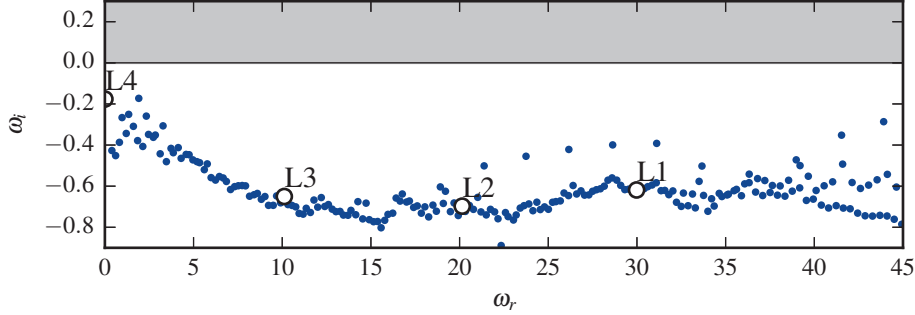
FIGURE 9. Low-frequency modes in the spectrum. The modes labelled L_1 - L_4 are depicted in figure 10, and the corresponding eigenvalues are \omega_{L_1} = 29.98 - 0.63i , \omega_{L_2} = 20.15 - 0.70i , \omega_{L_3} = 10.12 - 0.65i , \omega_{L_4} = 0.001 - 0.19i .
