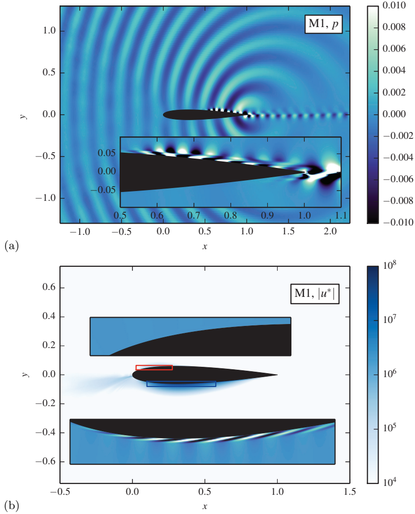
FIGURE 4. (a) Spatial structure of the global mode labelled M_1 , visualised by the real part of the associated near-field pressure levels, and the real part of the streamwise velocity levels in the vicinity of the airfoil surface (inset). The mode has been normalised by the maximum value of the velocity field in the near wake 1 < x < 1.2 . (b) Spatial structure of the associated adjoint global mode (labelled M_1 in figure 3), visualised by the magnitude of the streamwise velocity levels, and the real part in the insets.
