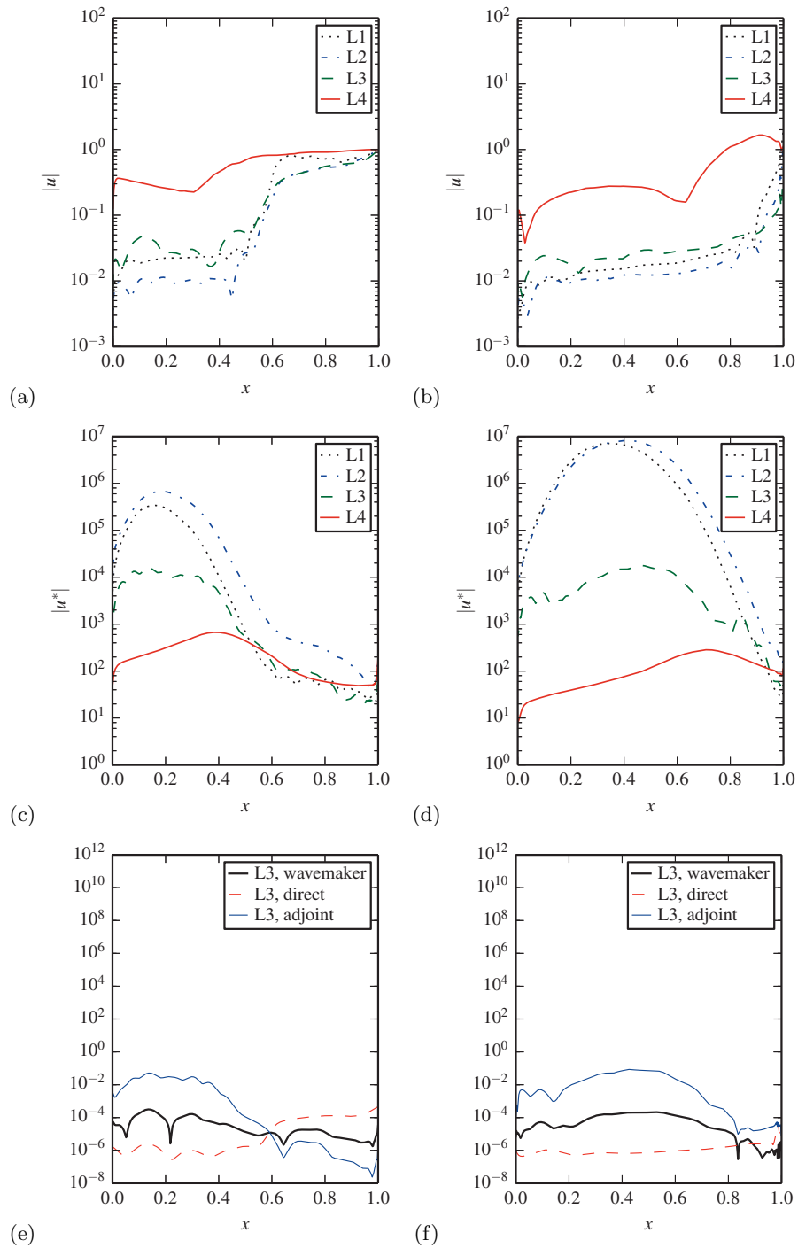
FIGURE 11. Evolution of the streamwise velocity peak along the aerofoil chord (a) on the suction- and (b) on the pressure surface of the aerofoil for the low-frequency modes labelled L 1 -L 4 in figure 9. (c,d) Same for the adjoint streamwise velocity peak. (e,f) Same for the direct mode, adjoint mode and wavemaker corresponding to L 3 .
