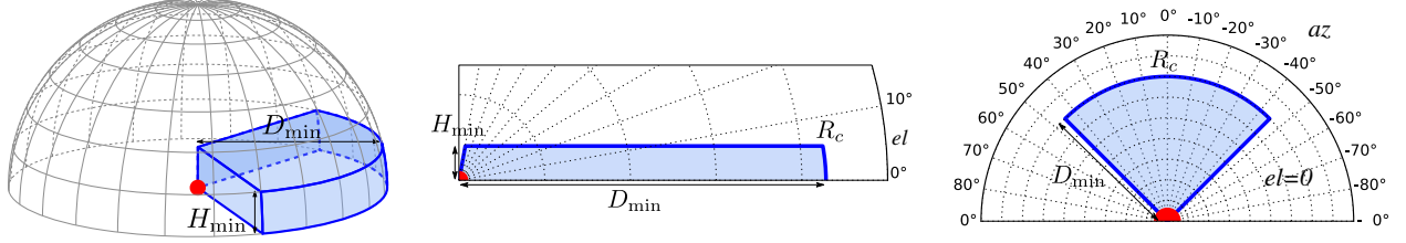
Fig. 2. Desired detection range (left), azimuth cut (center), elevation cut (right)
