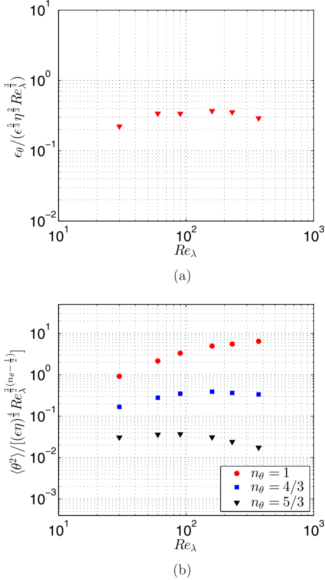
FIG. 5. (a) Reynolds-number dependence of the normalized dissipation of temperature fluctuations for Pr = 1 . (b) Variance of the temperature fluctuations, normalized assuming asymptotic scaling n_\theta = 5/3 or taking into account low-Reynolds-number corrections on the power-law exponent.
