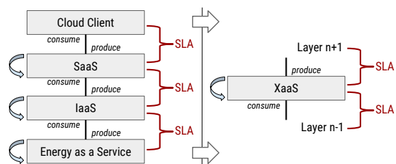
Figure 1: Specific Cloud layers vs. generic XaaS.
