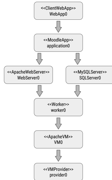
Figure 8: An initial configuration from our motivating example (SaaS level).
