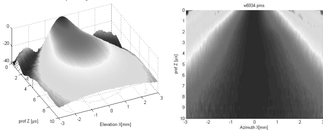
Fig. 6 : Radiation pattern with an excited representative element
