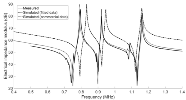
Fig. 3. Comparison of electrical impedances of ring 1 (solid line: experimental, dashed line: commercial data, dot line: adjusted data).
