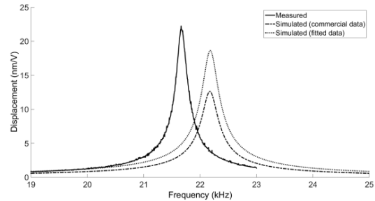
Fig. 5. Displacements at the center of the head mass of the BT:Co tonpilz (solid line: experimental, dashed line: commercial data, dot line: adjusted data).
