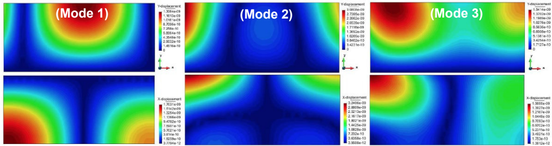
Fig. 2. Displacement fields (highest displacement in red and lowest displacement in blue) in a radial plane (y-direction for the thickness of the ring and x for the radial direction of the representative ring) for the three modes.
