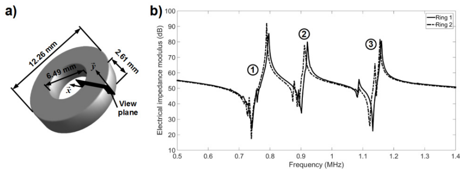
Fig. 1. (a) Geometrical dimensions of rings (b) electrical impedances of the two \text{BaTiO}_3\text{:Co} rings used for the Tonpilz fabrication.
