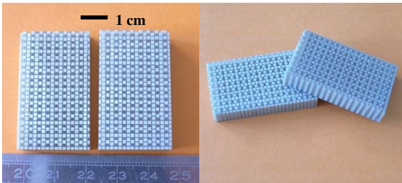
Fig. 4. Pictures of fabricated super-cell 1-3 piezocomposites.
