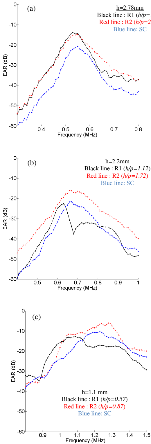
Fig. 5. Experimental electroacoustic responses (EAR) as a function of frequency for the three fabricated 1-3 piezocomposites (R1: regular with 2 mm pitch value, R2: regular with 1.33 pitch value, SC: super-cell): for a thickness of (a) 2.78 mm, (b) 2.2 mm and (c) 1.1 mm.
