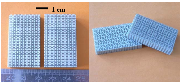
Fig. 4. Pictures of fabricated super-cell 1-3 piezocomposites.
