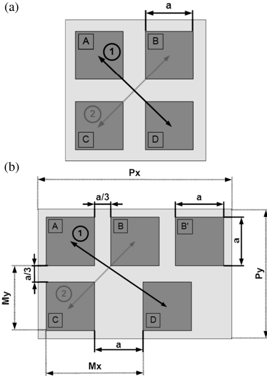
Fig. 1. Schematic representations (top views) of (a) regular and (b) super-cell structure for 1-3 piezocomposites (dark grey : piezoelectric rods, light grey : polymer).
