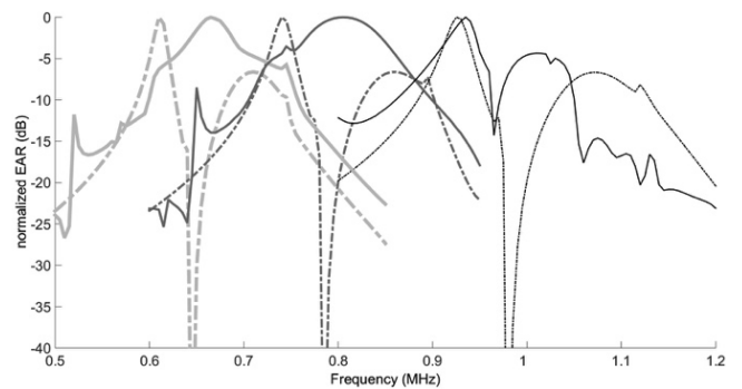
Fig. 2. Theoretical electroacoustic responses of the four piezocomposites for three different thicknesses: 1.33 mm (thick lines for configurations 1 and 2), 1.67 mm (medium line for configurations 1 and 3) and 2 mm (thin lines for configurations 1 and 4). Dashed line for regular and solid lines for super-cell structures.
