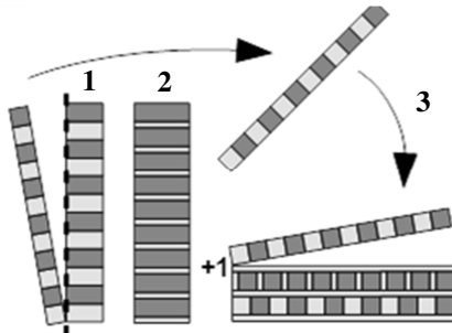
Fig. 3. Schematic representations (cross-sections) for the fabrication of the super-cell 1-3 piezocomposite.
