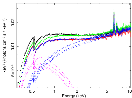
Fig. 4. Fit over the 0.3–10 keV energy range of the four 2014 XMM-Newton /pn spectra with the baseline Comptonization model (model \mathcal{B} ). The fit parameters are reported in Table 4. Black: March 18, red: March 20, green: March 22, and blue: March 24. Top panel : data and data/model ratio. Bottom panel : Unfolded spectra where the contribution of the model components are displayed. The following colour code for the emission components (dot-dashed curves) is used: magenta for the soft Comptonization (COMPTT), blue for the CUT-OFF POWER LAW (hot Comptonization). For clarity purposes, we have not displayed the Fe K line components.
