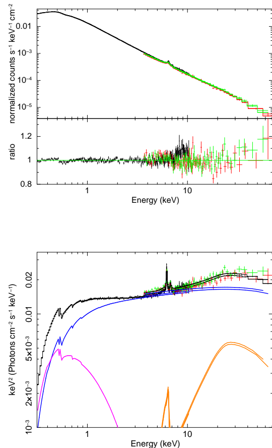
Fig. 9. Fit over the 0.3–79 keV energy range of the 2014 March 22 XMM-Newton /pn and NuSTAR data with model C , combining a soft Comptonization ( comptt ), a cut-off powerlaw, and a relativistic reflection component RELXILL (as produced by the cut-off power-law primary continuum shape). The corresponding fit parameters are reported in Table 7. Black: XMM-Newton /pn spectrum, red: NuSTAR FPMA, and green: NuSTAR FPMB. Top panel : data and data/model ratio. Bottom panel : Unfolded spectra where the contribution of the model components are displayed. The following colour code for the emission components (continuous lines) is used: magenta for COMPTT (soft Comptonization), blue for the CUT-OFF POWER LAW (hot Comptonization), orange for the relativistic reflection ( RELXILL ), and black for the total emission. For clarity purpose we have not displayed the total model and the three BLR Gaussian lines.
