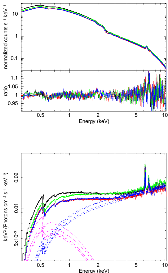
Fig. 4. Fit over the 0.3–10 keV energy range of the four 2014 XMM-Newton/pn spectra with the baseline Comptonization model (model \mathcal{B} ). The fit parameters are reported in Table 4. Black: March 18, red: March 20, green: March 22, and blue: March 24. Top panel: data and data/model ratio. Bottom panel: Unfolded spectra where the contribution of the model components are displayed. The following colour code for the emission components (dot-dashed curves) is used: magenta for the soft Comptonization (COMPTT), blue for the CUT-OFF POWER LAW (hot Comptonization). For clarity purposes, we have not displayed the Fe K line components.
