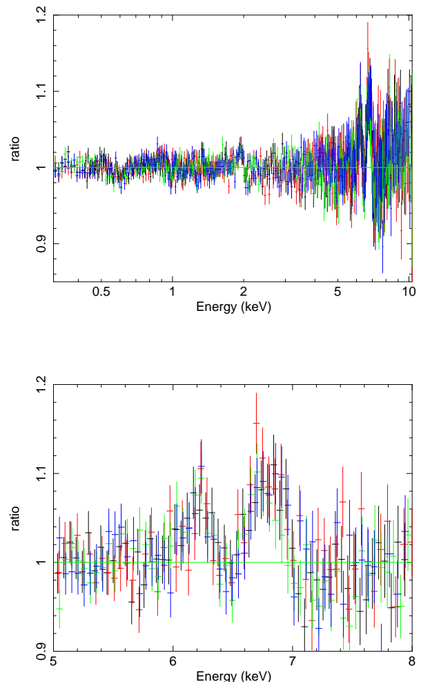
Fig. 3. Data/model ratio of the fit over the 0.3–10 keV energy range of the four 2014 XMM-Newton/pn spectra with the baseline relativistic reflection model (model \mathcal{A} ). The best fit parameters are reported in Table 3. Black: March 18, red: March 20, green: March 22, and blue: March 24. Top panel: The full 0.3–10 keV energy range. Bottom panel: Zoom on the Fe K\alpha complex.
