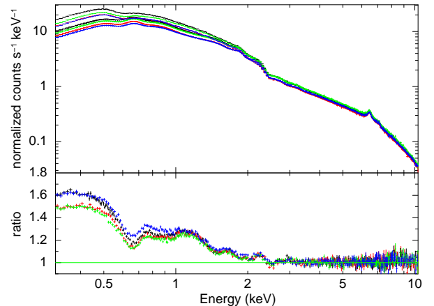
Fig. 2. Extrapolation down to 0.3 keV of the fit over the 3–10 keV energy range of the four 2014 XMM-Newton /pn spectra with the baseline relativistic reflection model (model \mathcal{A} ), where q is allowed to vary and R_{\text{in}} is fixed to the ISCO. The fit parameters are reported in Table 2 (column 2). Black: March 18, red: March 20, green: March 22, and blue: March 24.
