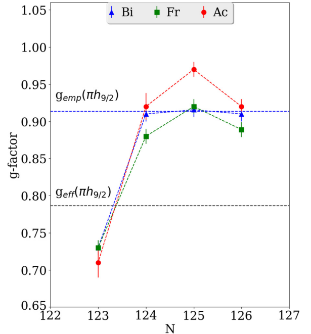
FIG. 9. Comparison between the g factors for the actinium isotopes with isotopes of francium and bismuth. The g_{\text{eff}} is the Schmidt value typical for this region [43]. The blue dashed line corresponds to the empirical g -factor value from ^{209}\text{Bi} [51]. Here, only the statistical errors are shown.
