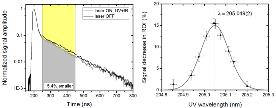
Fig. 4. Spectroscopy of Ps 1 \rightarrow 3 transition.
