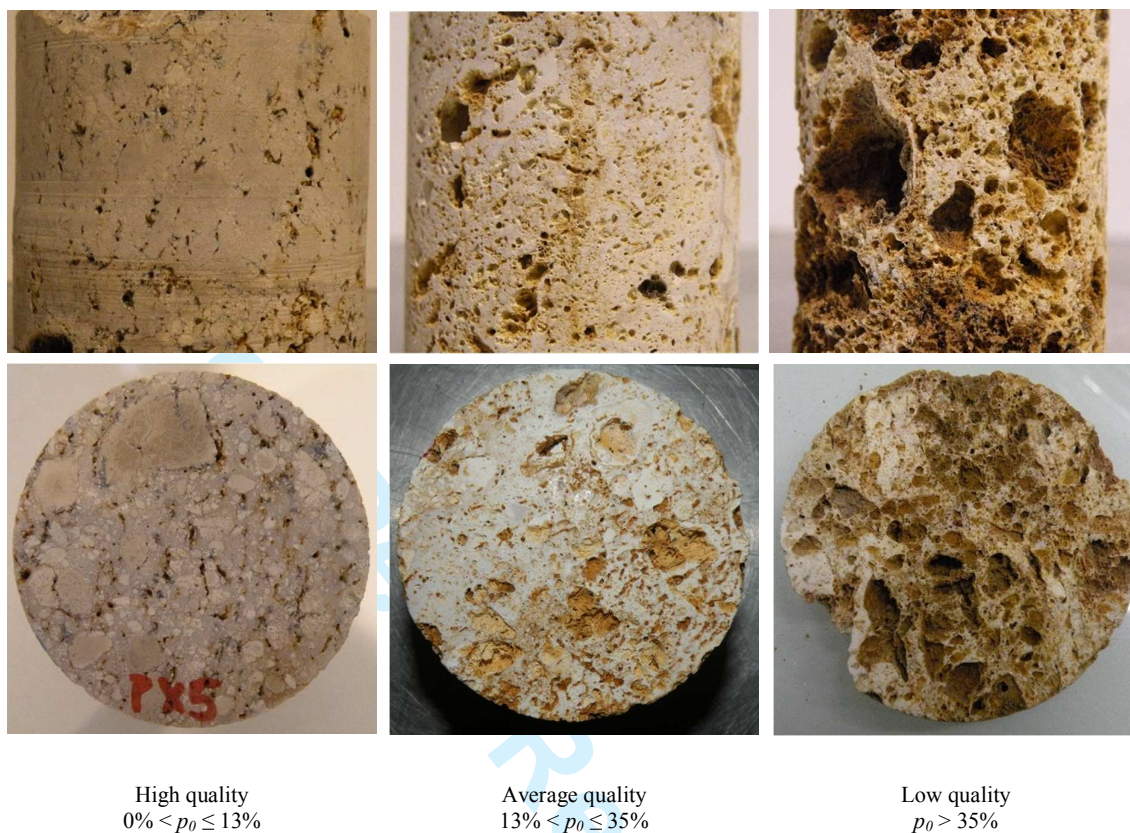
Fig. 14 Observed composition of different types of Millstone and proposed classification regarding its porosity p_0
