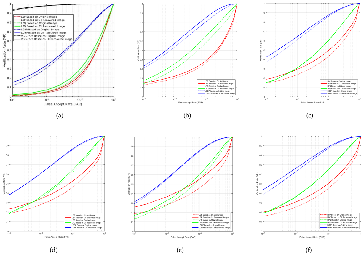
Fig. 11. Several ROC curves for different gray-scale methods. (a) No gray-scale method, (b) GRF, (c) DOG, (d) WEB, (e) SGL, (f) TT. Note that only (a) contains ROC curves for the VGG-Face model as it requires RGB images as model input.
