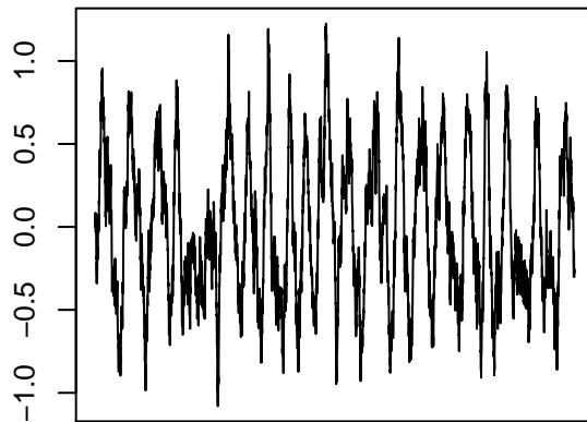
Channel kinetic
