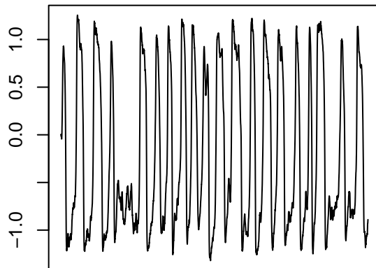
Membrane potential
