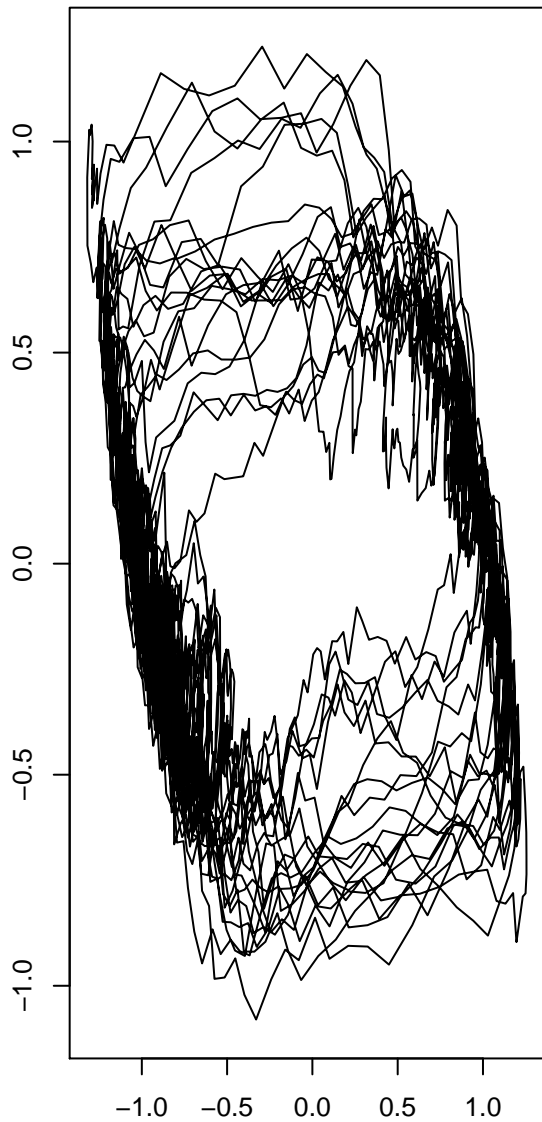
Phase portrait
