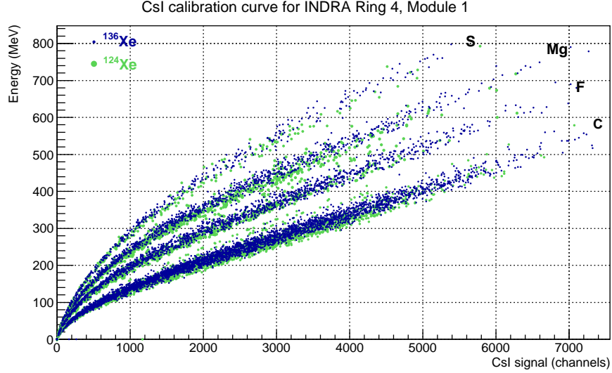
Figure 2: Energy ( E_0 ) - Light ( \mathcal{L} ) correlation in the CsI(Tl) scintillator of telescope 1 of the ring 4 ( 7^\circ \leq \theta \leq 10^\circ ), shown here for the two systems ^{124}\text{Xe} + ^{112}\text{Sn} and ^{136}\text{Xe} + ^{124}\text{Sn} at 32A MeV, and for some selected elements: carbon, fluorine, magnesium and sulphur. The large/green symbols correspond to the (n)-poor system ( ^{124}\text{Xe} + ^{112}\text{Sn} ) and the small/blue ones to the (n)-rich system ( ^{136}\text{Xe} + ^{124}\text{Sn} ).
