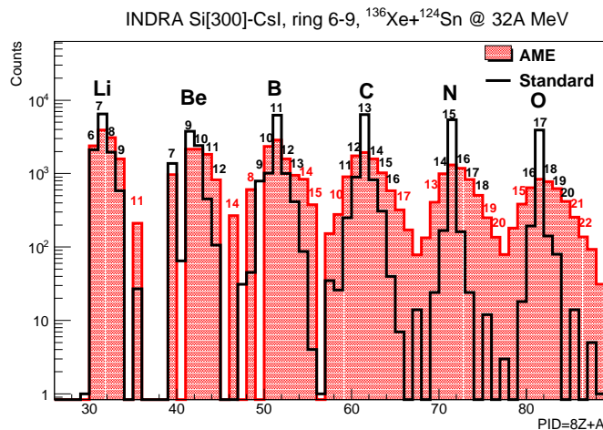
Figure 4: Isotopic distributions from lithium (left) to oxygen (right). The isotopes are indicated by their mass numbers. The black and grey/red labels are explained in the text. Data concern the rings 6 to 9 for the system ^{136}\text{Xe} + ^{124}\text{Sn} system at 32A MeV recorded with INDRA and correspond to forward angles between 14^\circ and 45^\circ in laboratory frame. Empty histograms are the results obtained with the standard \Delta E - \mathcal{L} method and filled histograms those from the AME method for the same sample of events. The Silicon stage is 300 \mu\text{m} thick.
