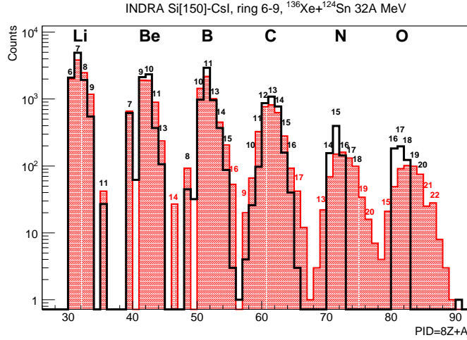
Figure 5: Isotopic distributions from lithium (left) to oxygen (right). The isotopes are indicated by their mass numbers. The black and grey/red labels are explained in the text. Data concern the specific telescopes with a high gain 150 \mu\text{m} Silicon from rings 6 to 9 for the system ^{136}\text{Xe} + ^{124}\text{Sn} at 32A MeV recorded with INDRA and correspond to forward angles between 14^\circ and 45^\circ in the laboratory frame. Empty histograms are the results obtained with the standard \Delta E - \mathcal{L} method and filled histograms those from the AME method for the same sample of events.
