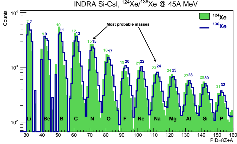
Figure 6: Isotopic distributions (PID as 8Z + A ) from lithium (left) to phosphorus isotopes (right), provided by AME with ordinary telescopes ( 300 \mu\text{m} -thick Si). The filled histograms correspond to the ^{124}\text{Xe} + ^{112}\text{Sn} system and the empty histograms to the ^{136}\text{Xe} + ^{124}\text{Sn} system at the same incident energy per nucleon E/A = 45 \text{ MeV} ( INDRA data). The most abundant isotope in each case is indicated too.
