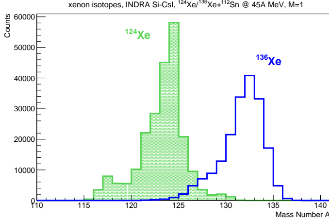
Figure 9: INDRA data. Isotopic distribution of xenon isotopes ( Z = 54 ) for the ^{124}\text{Xe} + ^{112}\text{Sn} (filled histogram) and ^{136}\text{Xe} + ^{112}\text{Sn} (empty histogram) at 45A MeV provided by the AME method, in the most forward rings (1-3) for a trigger multiplicity M = 1 .
