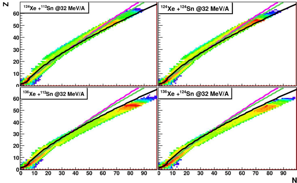
Figure 10: Z - N charts of the detected nuclei in the forward rings (1-9) of INDRA for a trigger multiplicity M \geq 4 from the four reactions ^{136,124}\text{Xe} + ^{112,124}\text{Sn} at 32A MeV. Data correspond to the AME method. The different grey/coloured curves correspond to the EAL hypotheses on the neutron number N and the black line to the \beta -stability valley one. See text for explanation.
