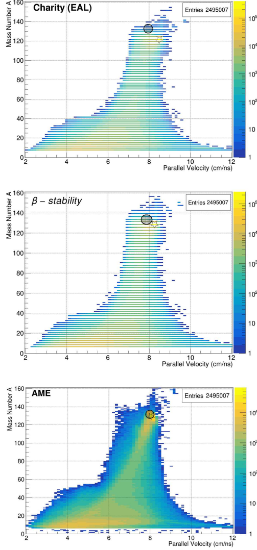
Figure 7: INDRA data. Correlation between the velocity V_z in cm/ns, parallel to the beam direction, and the atomic mass A for ^{136}\text{Xe} + ^{112}\text{Sn} at 32A MeV obtained in the very forward rings (1-5) for a trigger multiplicity M \geq 1 . The upper panel displays the traditional \Delta E - \mathcal{L} identification method with no mass determination and the EAL hypothesis for the masses of the fragments. The same for the middle panel, but with the \beta -stability valley hypothesis for the masses of the fragments. In the lower panel are plotted the results obtained with the new AME method. The circles indicate the projectile mass ( A = 136 ) and the parallel projectile velocity ( V_z = 7.9 cm/ns), while the stars correspond to the peak of each two-dimensional distribution.
