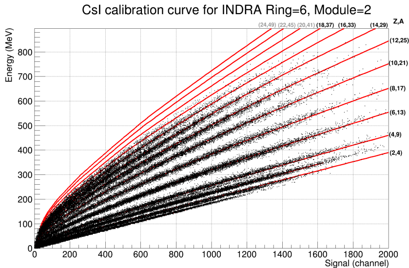
Figure 1: Energy ( E_0 ) - Light ( \mathcal{L} ) correlation in a CsI( Tl ) scintillator, for even- Z fragments. The points correspond to data from the telescope 2 of the ring 6 ( 14^\circ \leq \theta \leq 20^\circ ) of the INDRA 4\pi array for the system ^{136}\text{Xe} + ^{124}\text{Sn} at 32A MeV. The atomic number of the heaviest fragments emitted in this angular domain is Z = 16 . The full/coloured lines illustrate the Eq. (3) predictions. The mass number for each element is likely corresponding to the most probable isotope, here A = 2Z + 1 . See text for explanation.
