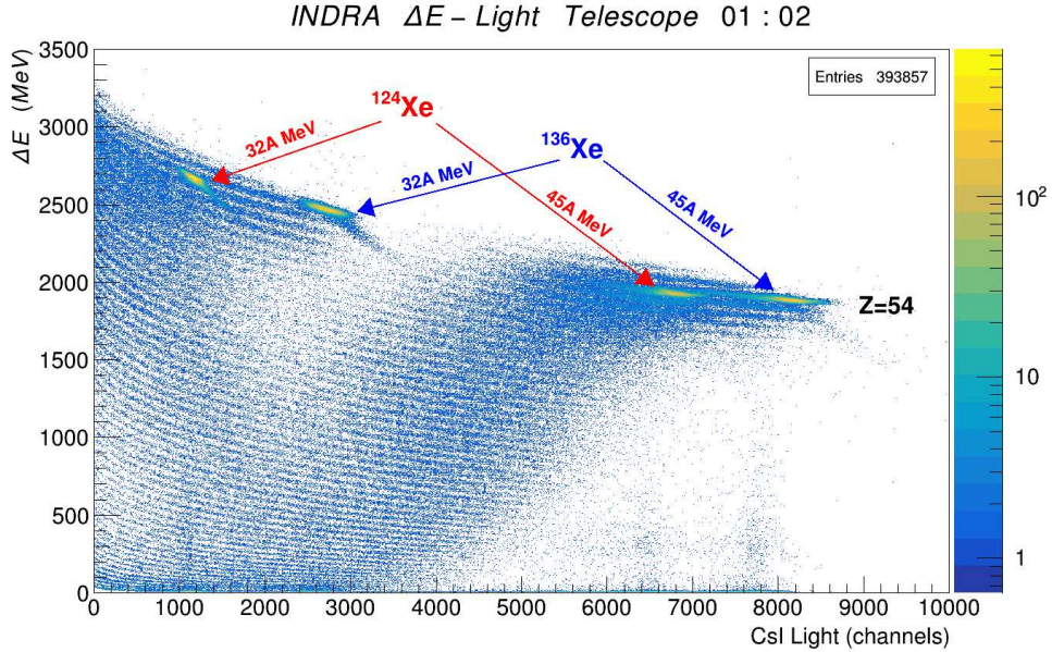
Figure 3: \Delta E - \mathcal{L} correlation for INDRA data obtained with a module placed at a forward angle for the ^{124,136}\text{Xe} + ^{124}\text{Sn} systems at 32A MeV and 45A MeV bombarding energies, illustrating its sensitivity to the detected fragment mass. The Silicon stage is 300 \mu\text{m} thick. See text for explanation.
