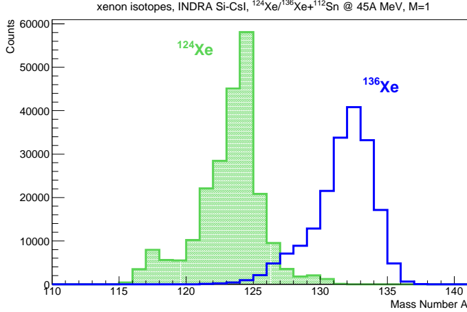
Figure 9: INDRA data. Isotopic distribution of xenon isotopes ( Z = 54 ) for the ^{124}\text{Xe}+^{112}\text{Sn} (filled histogram) and ^{136}\text{Xe}+^{112}\text{Sn} (empty histogram) at 45A MeV provided by the AME method, in the most forward rings (1-3) for a trigger multiplicity M = 1 .
