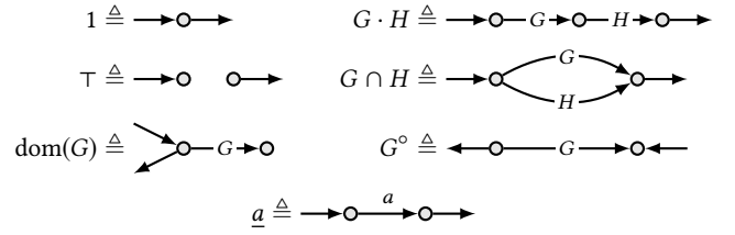
Figure 2. Graph operations.
