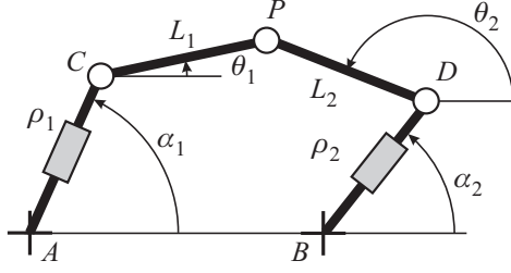
Figure 2: Two degree-of-freedom parallel mechanism
