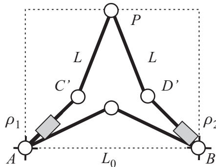
Figure 12: The orthoglide mechanism
