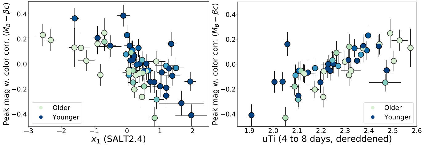
Fig. 12. Comparing peak SN magnitude (including color correction) with SALT2.4 x_1 ( left panel ) and uTi ( right panel ). Lighter shaded points were found in R17 to originate in locally passive regions, and likely from old progenitors, while dark blue points were found in regions dominated by star formation. These are separated in x_1 (left), but not in uTi (right).
